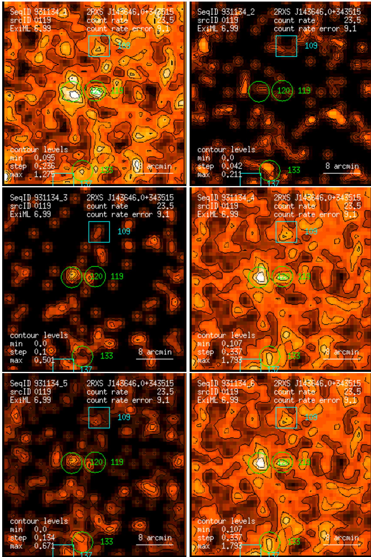
Figure 119: RASS 931134: detection 0119: band rate images, Gaussian filter: (1) PSPC channels 11 – 41, (2) 52 – 90, (3) 91 – 201, (4) 11 – 235, (5) 52 – 201, (6) 11 – 201. Broad band rates in counts/ks. Band rate contour levels in counts/ks/arcmin 2 .
