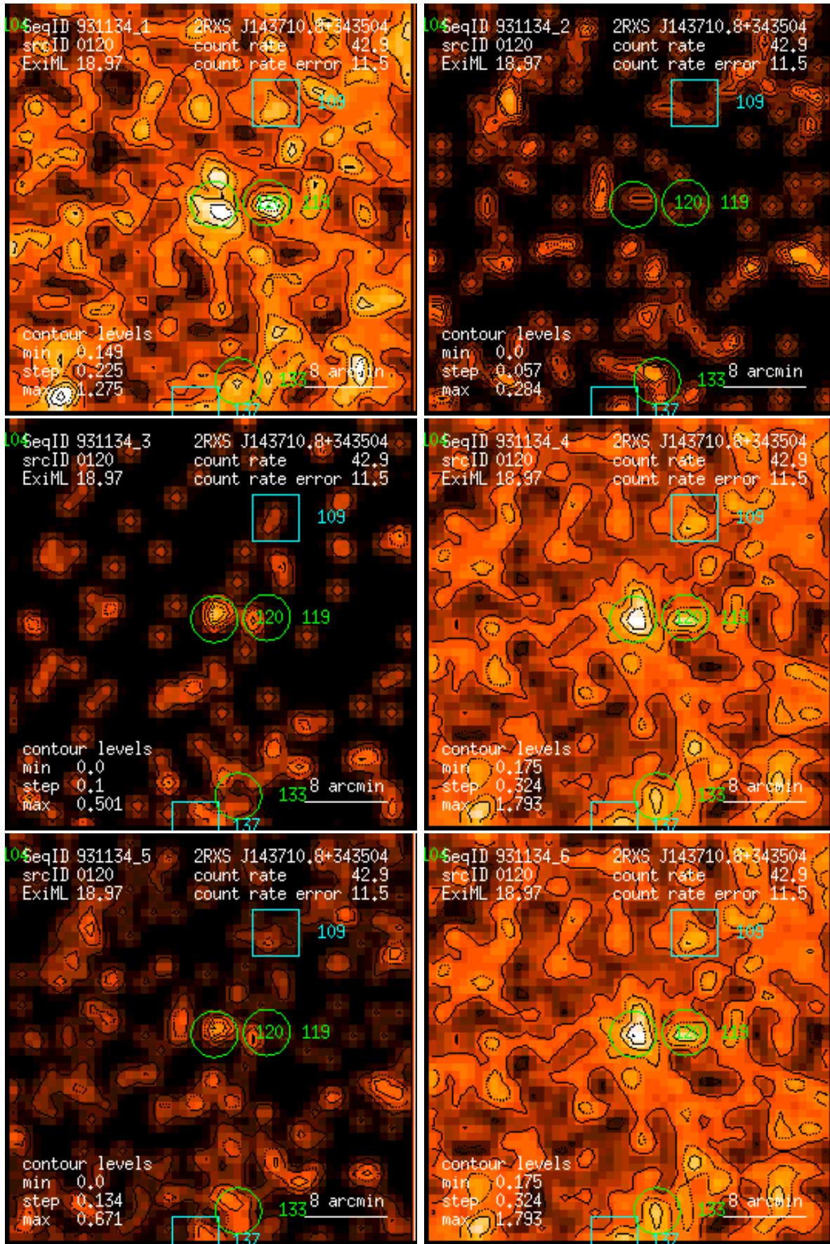
Figure 120: RASS 931134: detection 0120: band rate images, Gaussian filter: (1) PSPC channels 11 – 41, (2) 52 – 90, (3) 91 – 201, (4) 11 – 235, (5) 52 – 201, (6) 11 – 201. Broad band rates in counts/ks. Band rate contour levels in counts/ks/arcmin 2 .
