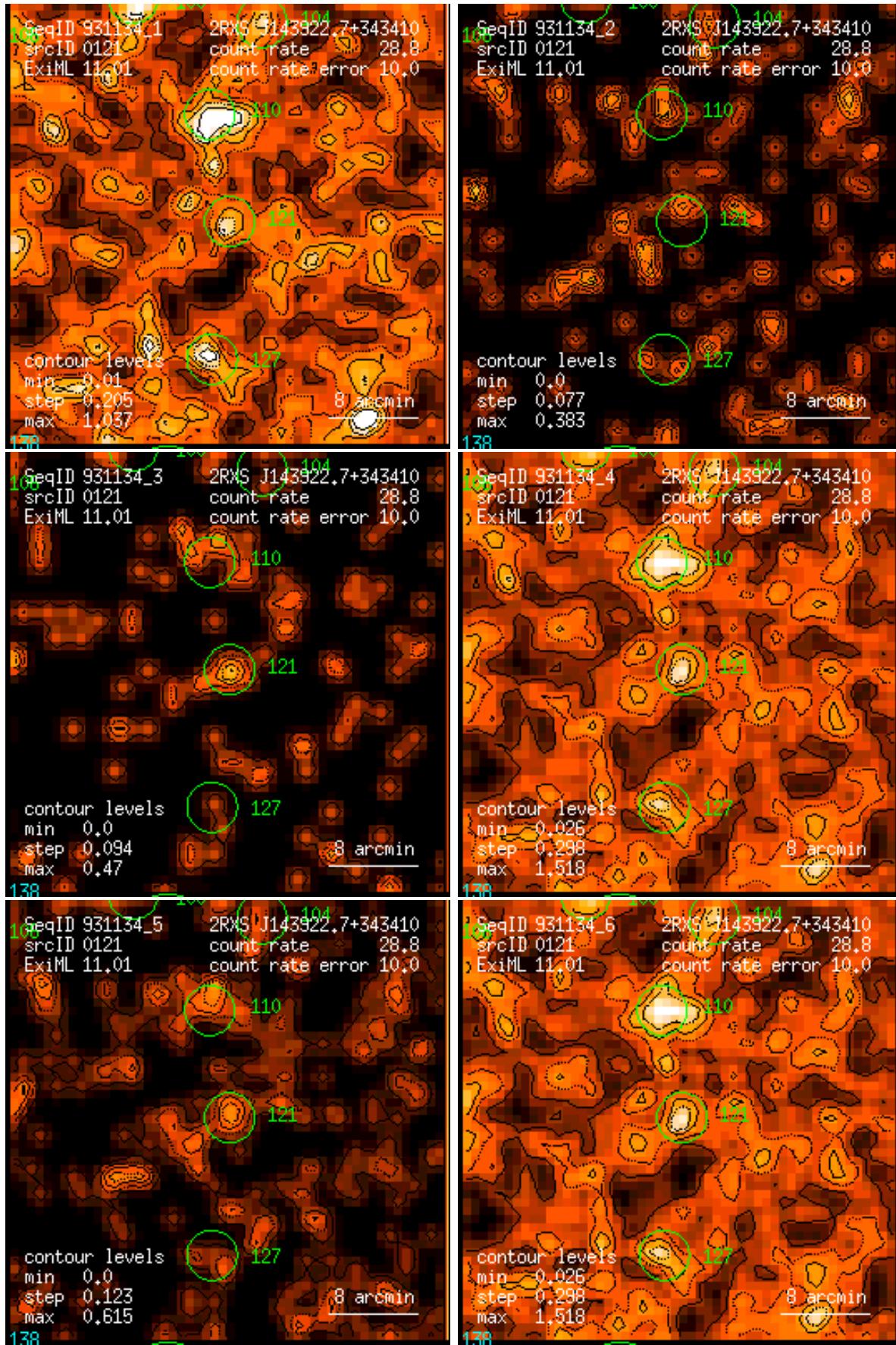
Figure 121: RASS 931134: detection 0121: band rate images, Gaussian filter: (1) PSPC channels 11 – 41, (2) 52 – 90, (3) 91 – 201, (4) 11 – 235, (5) 52 – 201, (6) 11 – 201. Broad band rates in counts/ks. Band rate contour levels in counts/ks/arcmin 2 .
