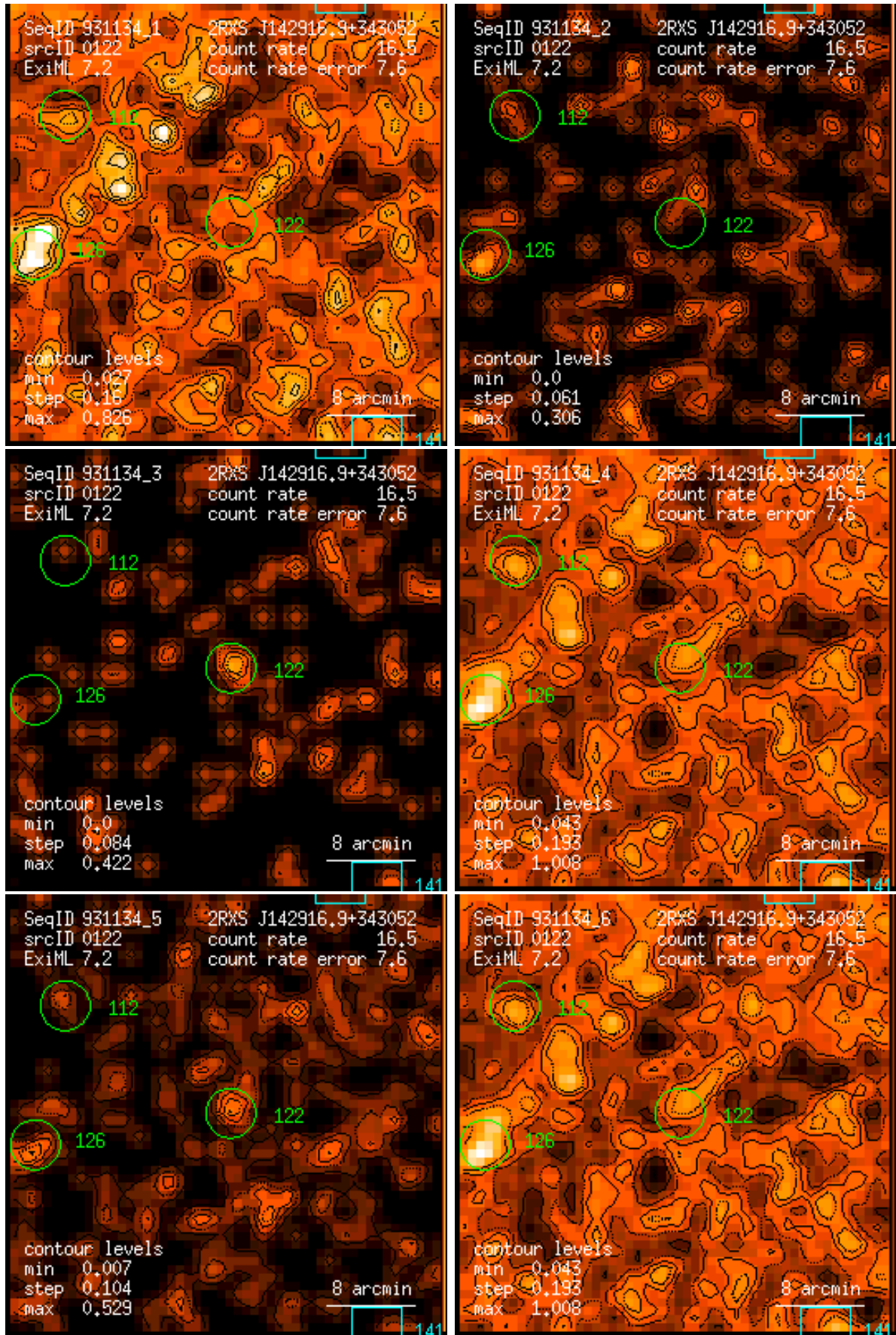
Figure 122: RASS 931134: detection 0122: band rate images, Gaussian filter: (1) PSPC channels 11 – 41, (2) 52 – 90, (3) 91 – 201, (4) 11 – 235, (5) 52 – 201, (6) 11 – 201. Broad band rates in counts/ks. Band rate contour levels in counts/ks/arcmin 2 .
