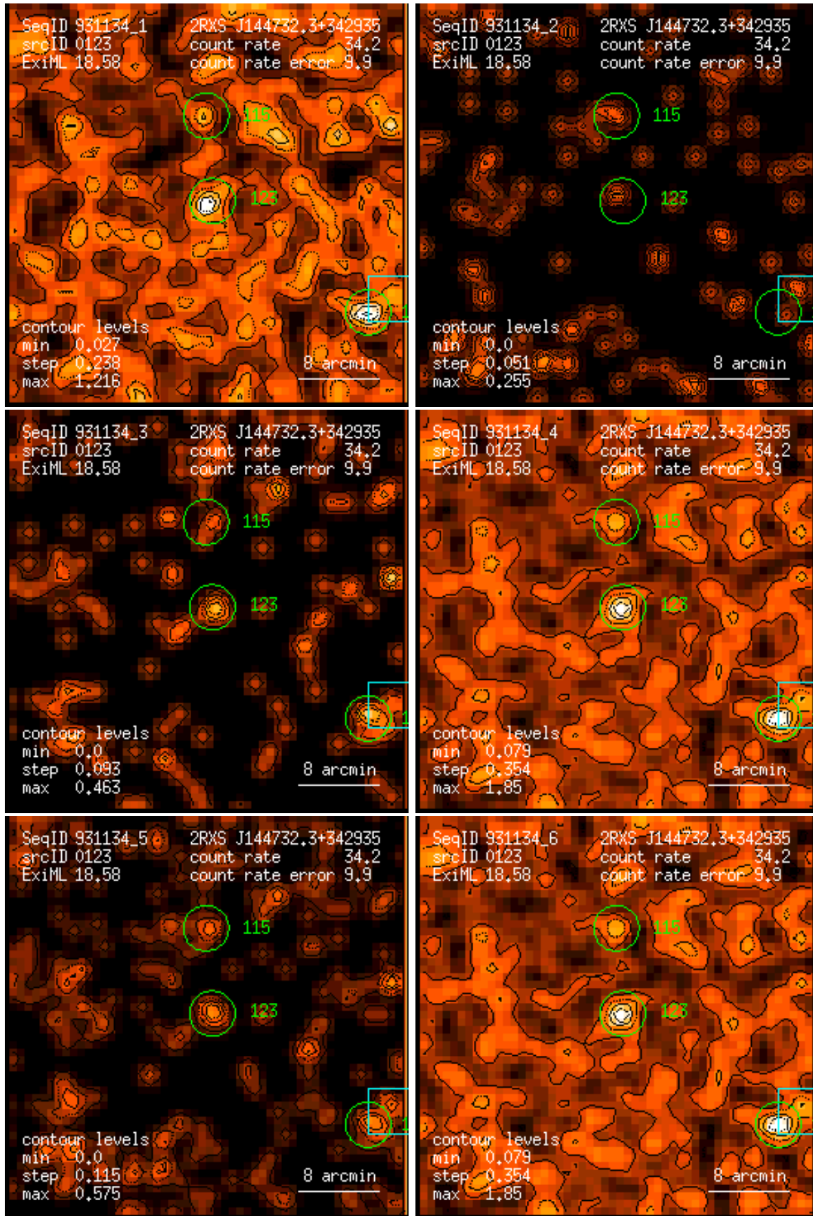
Figure 123: RASS 931134: detection 0123: band rate images, Gaussian filter: (1) PSPC channels 11 – 41, (2) 52 – 90, (3) 91 – 201, (4) 11 – 235, (5) 52 – 201, (6) 11 – 201. Broad band rates in counts/ks. Band rate contour levels in counts/ks/arcmin 2 .
