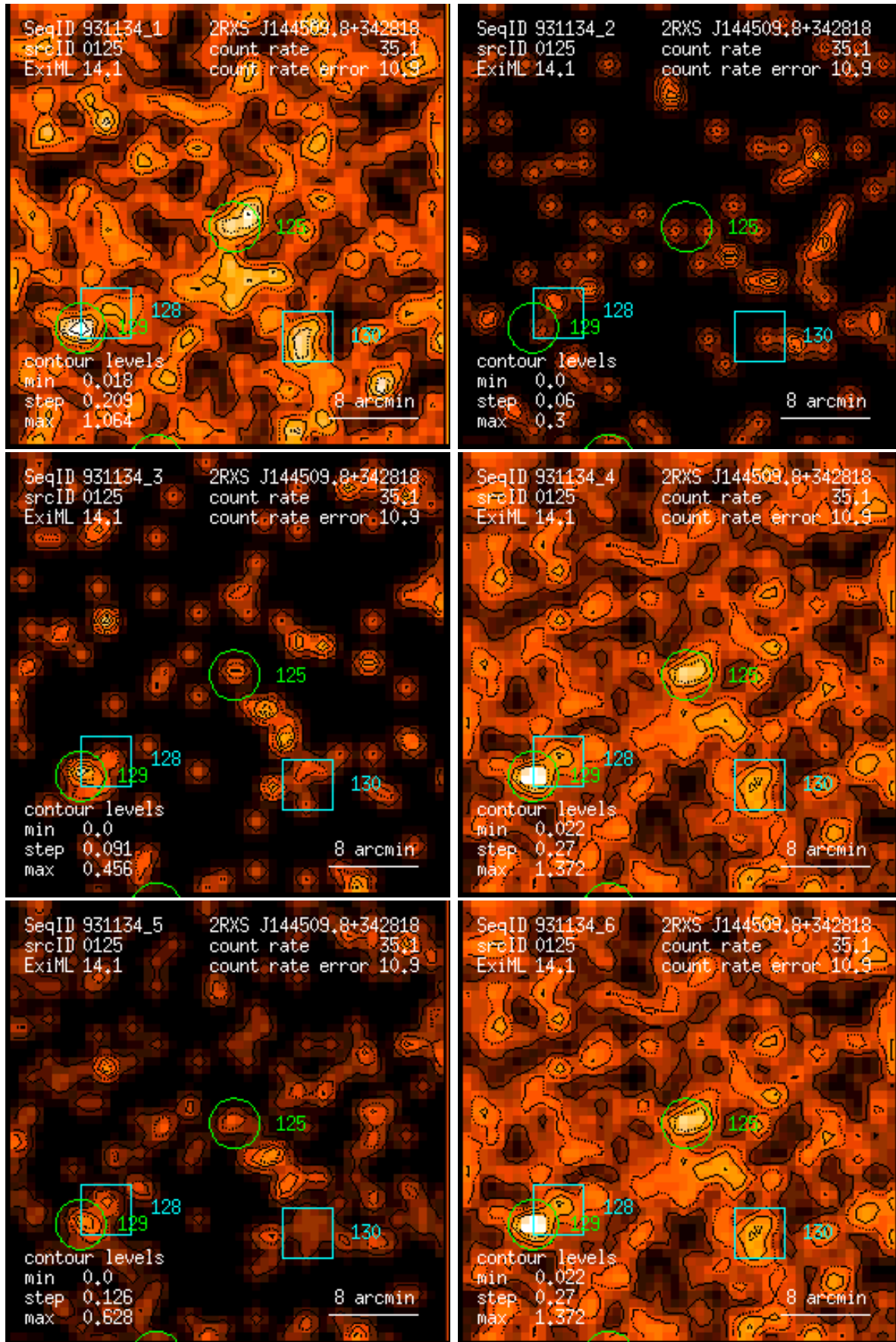
Figure 125: RASS 931134: detection 0125: band rate images, Gaussian filter: (1) PSPC channels 11 – 41, (2) 52 – 90, (3) 91 – 201, (4) 11 – 235, (5) 52 – 201, (6) 11 – 201. Broad band rates in counts/ks. Band rate contour levels in counts/ks/arcmin 2 .
