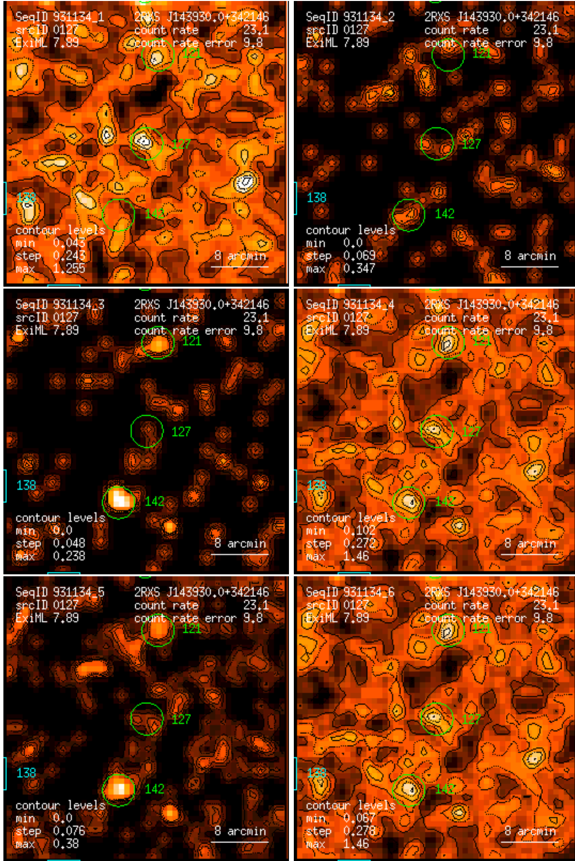
Figure 127: RASS 931134: detection 0127: band rate images, Gaussian filter: (1) PSPC channels 11 – 41, (2) 52 – 90, (3) 91 – 201, (4) 11 – 235, (5) 52 – 201, (6) 11 – 201. Broad band rates in counts/ks. Band rate contour levels in counts/ks/arcmin 2 .
