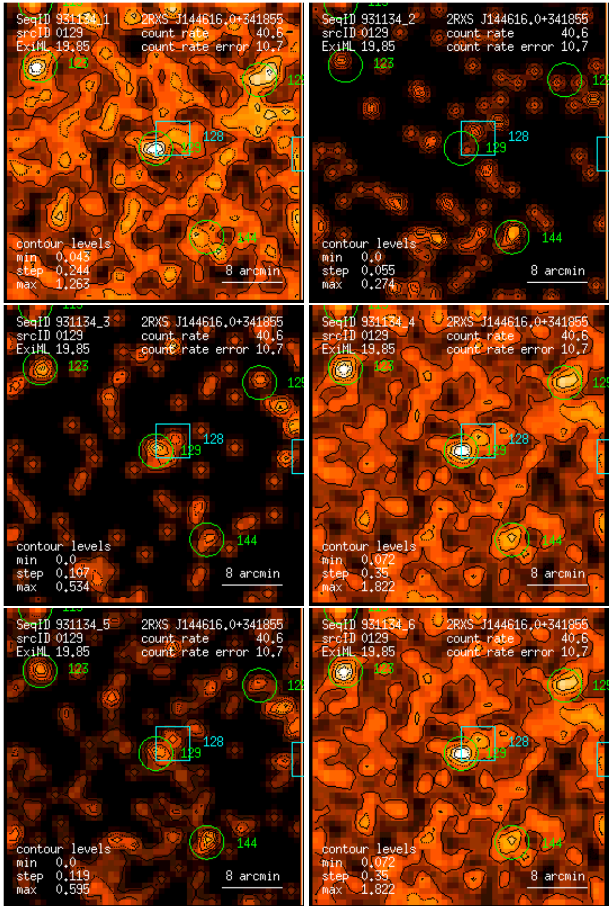
Figure 129: RASS 931134: detection 0129: band rate images, Gaussian filter: (1) PSPC channels 11 – 41, (2) 52 – 90, (3) 91 – 201, (4) 11 – 235, (5) 52 – 201, (6) 11 – 201. Broad band rates in counts/ks. Band rate contour levels in counts/ks/arcmin 2 .
