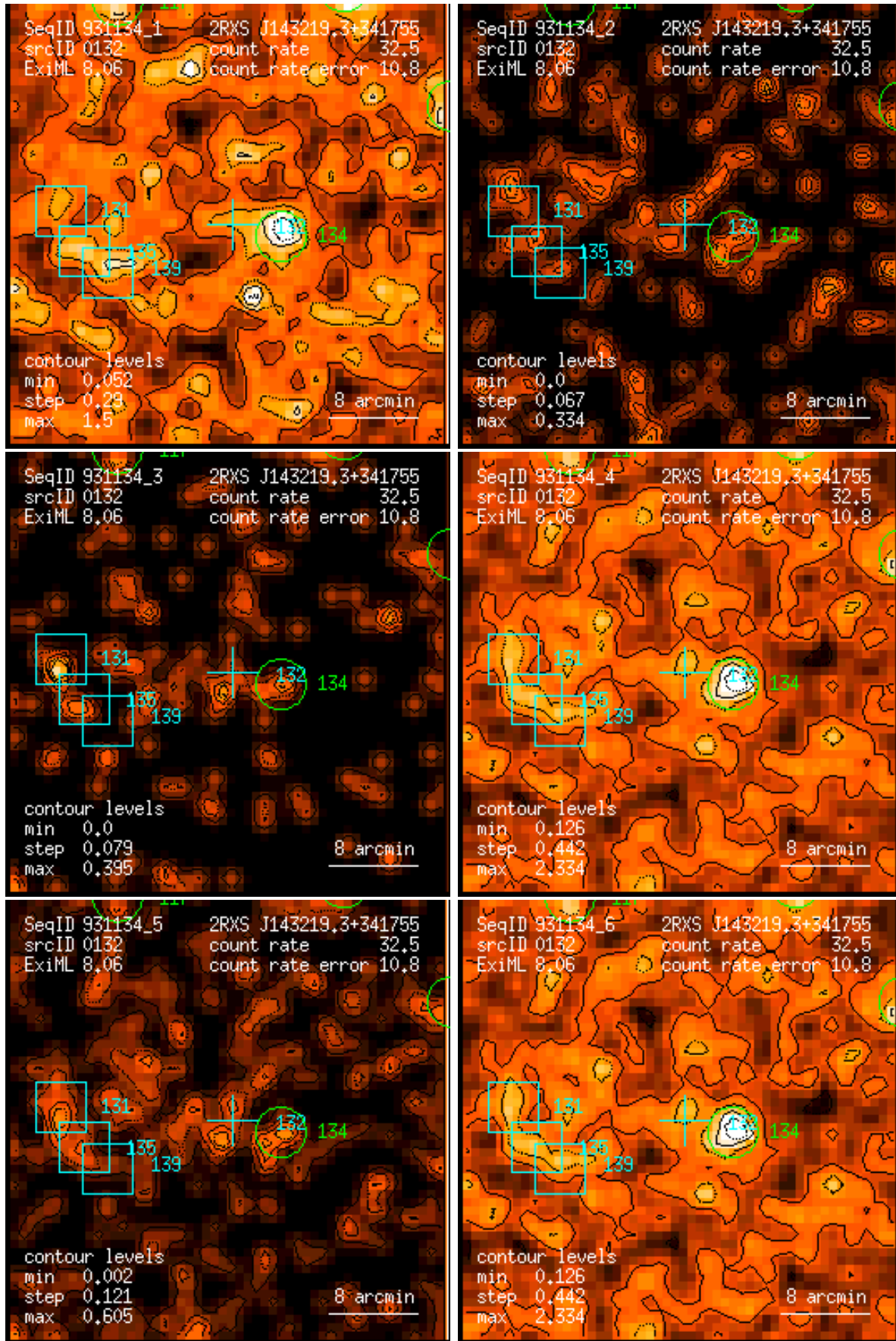
Figure 132: RASS 931134: detection 0132: band rate images, Gaussian filter: (1) PSPC channels 11 – 41, (2) 52 – 90, (3) 91 – 201, (4) 11 – 235, (5) 52 – 201, (6) 11 – 201. Broad band rates in counts/ks. Band rate contour levels in counts/ks/arcmin 2 .
