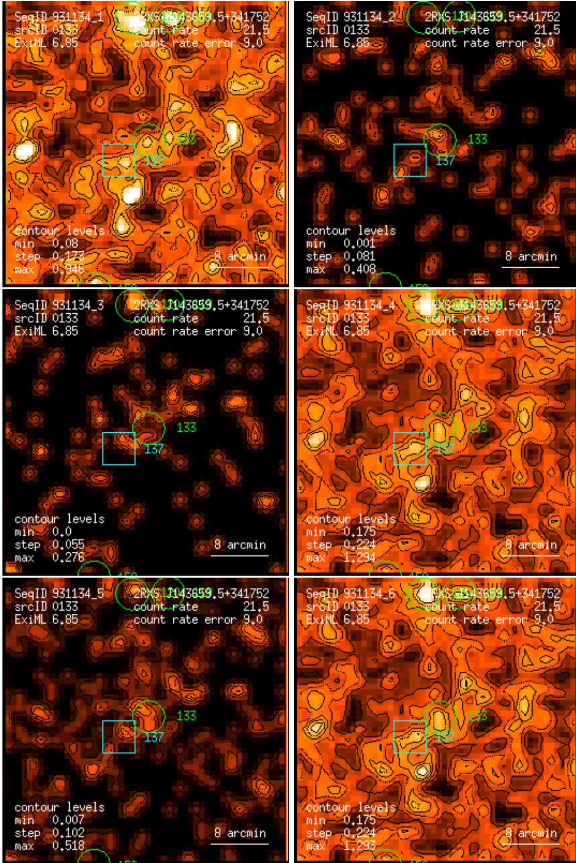
Figure 133: RASS 931134: detection 0133: band rate images, Gaussian filter: (1) PSPC channels 11 – 41, (2) 52 – 90, (3) 91 – 201, (4) 11 – 235, (5) 52 – 201, (6) 11 – 201. Broad band rates in counts/ks. Band rate contour levels in counts/ks/arcmin 2 .
