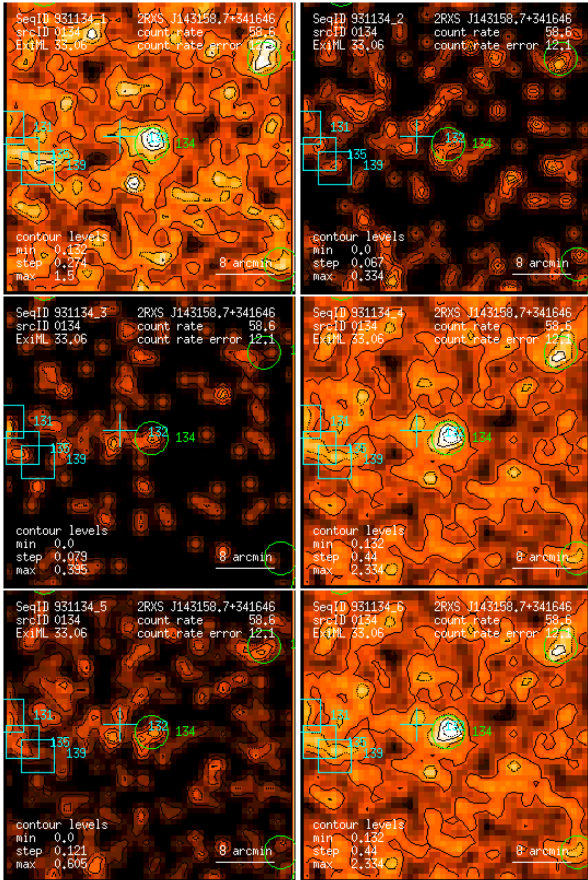
Figure 134: RASS 931134: detection 0134: band rate images, Gaussian filter: (1) PSPC channels 11 – 41, (2) 52 – 90, (3) 91 – 201, (4) 11 – 235, (5) 52 – 201, (6) 11 – 201. Broad band rates in counts/ks. Band rate contour levels in counts/ks/arcmin 2 .
