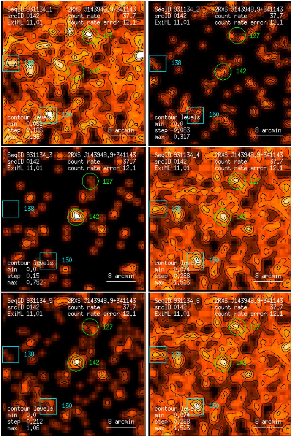
Figure 142: RASS 931134: detection 0142: band rate images, Gaussian filter: (1) PSPC channels 11 – 41, (2) 52 – 90, (3) 91 – 201, (4) 11 – 235, (5) 52 – 201, (6) 11 – 201. Broad band rates in counts/ks. Band rate contour levels in counts/ks/arcmin 2 .
