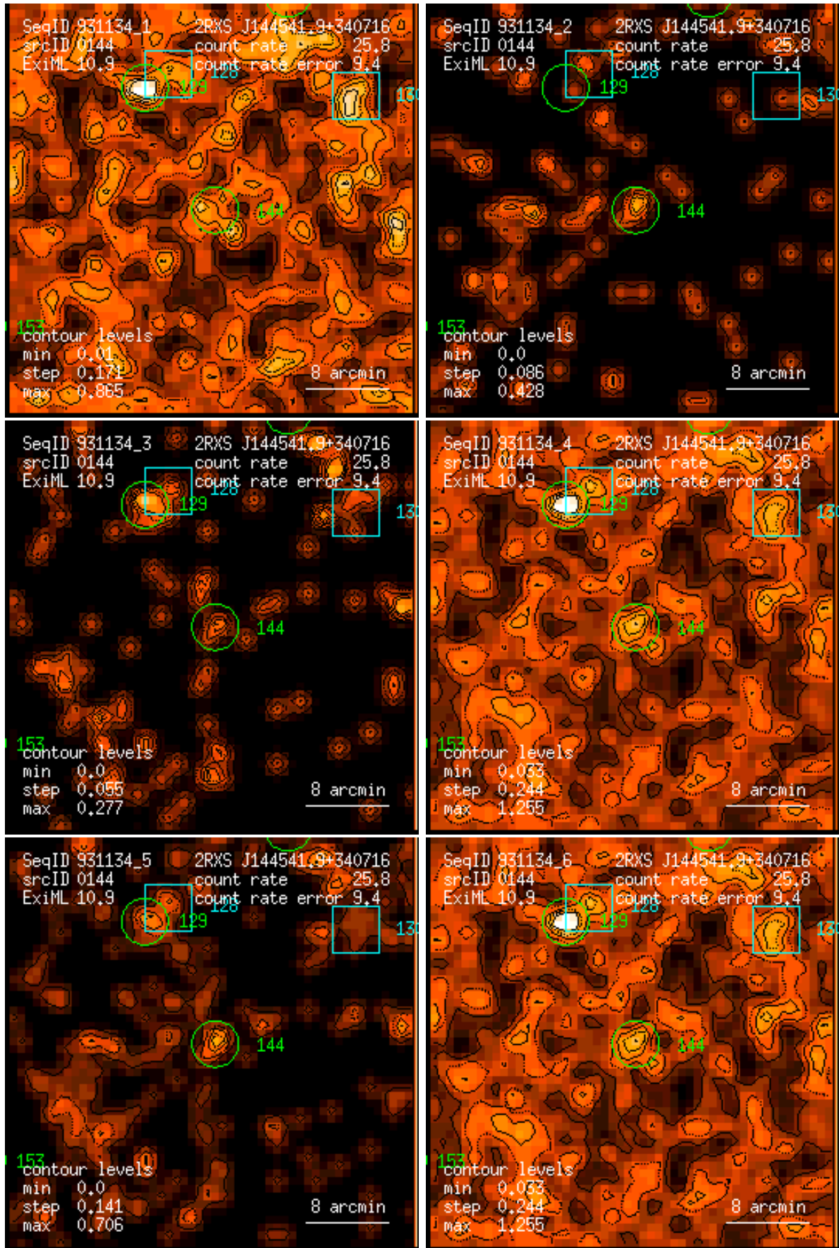
Figure 144: RASS 931134: detection 0144: band rate images, Gaussian filter: (1) PSPC channels 11 – 41, (2) 52 – 90, (3) 91 – 201, (4) 11 – 235, (5) 52 – 201, (6) 11 – 201. Broad band rates in counts/ks. Band rate contour levels in counts/ks/arcmin 2 .
