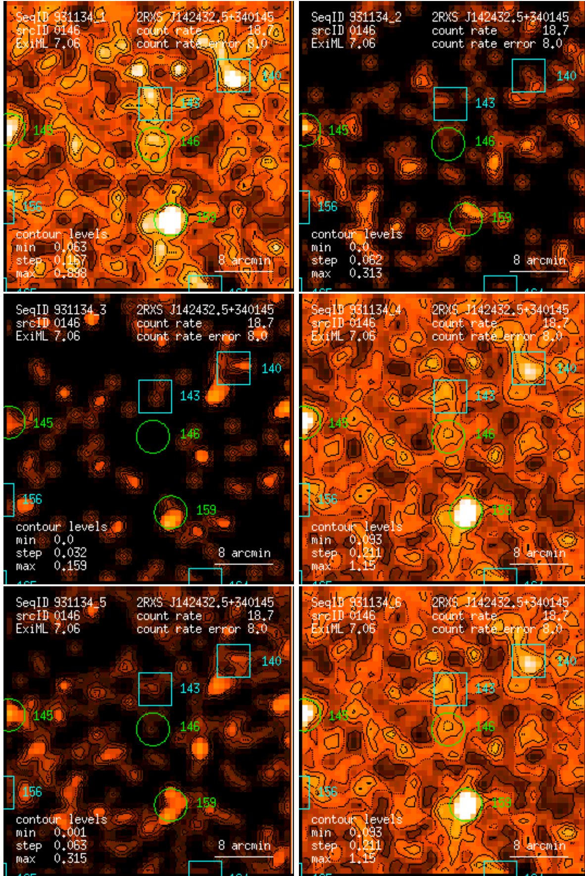
Figure 146: RASS 931134: detection 0146: band rate images, Gaussian filter: (1) PSPC channels 11 – 41, (2) 52 – 90, (3) 91 – 201, (4) 11 – 235, (5) 52 – 201, (6) 11 – 201. Broad band rates in counts/ks. Band rate contour levels in counts/ks/arcmin 2 .
