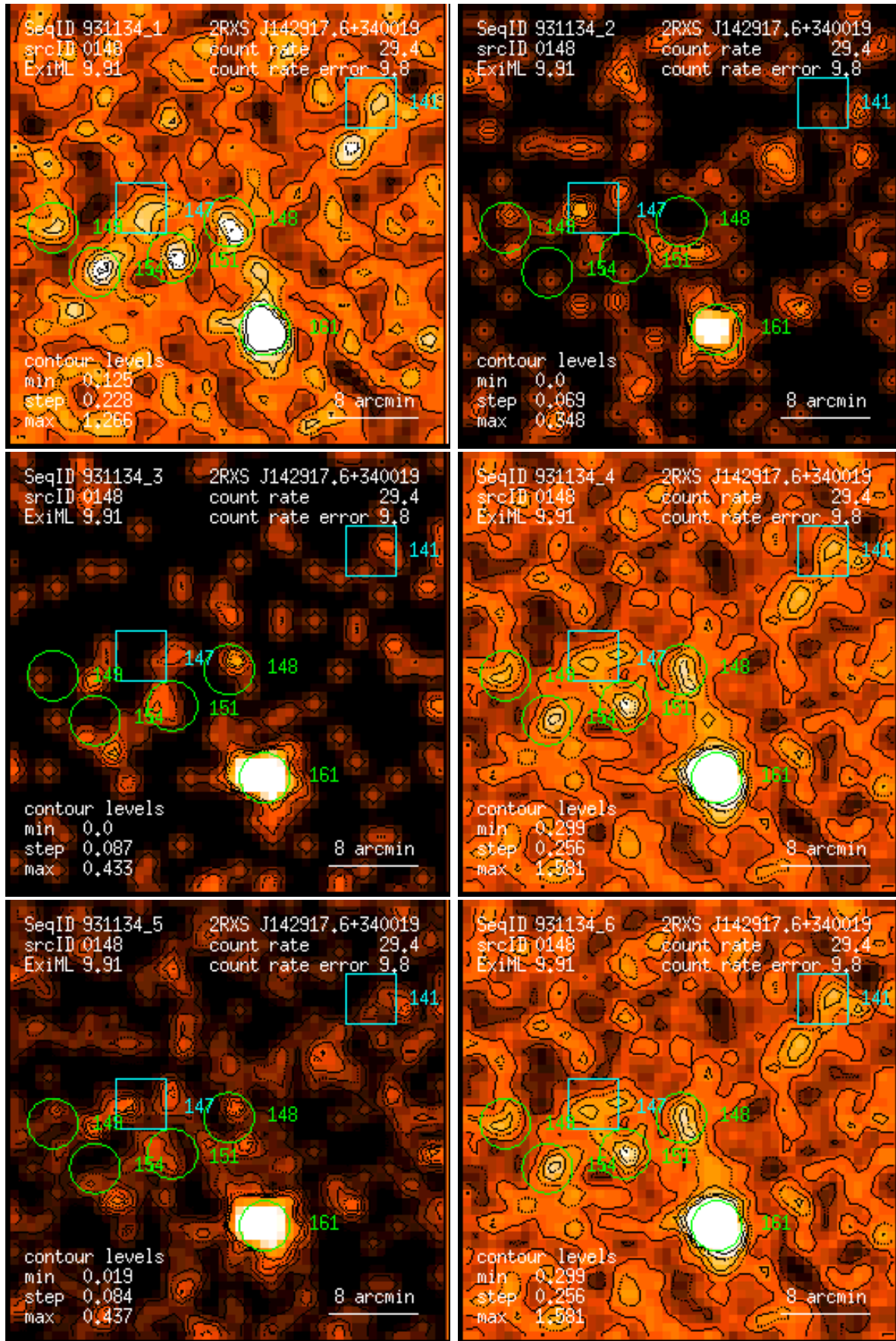
Figure 148: RASS 931134: detection 0148: band rate images, Gaussian filter: (1) PSPC channels 11 – 41, (2) 52 – 90, (3) 91 – 201, (4) 11 – 235, (5) 52 – 201, (6) 11 – 201. Broad band rates in counts/ks. Band rate contour levels in counts/ks/arcmin 2 .
