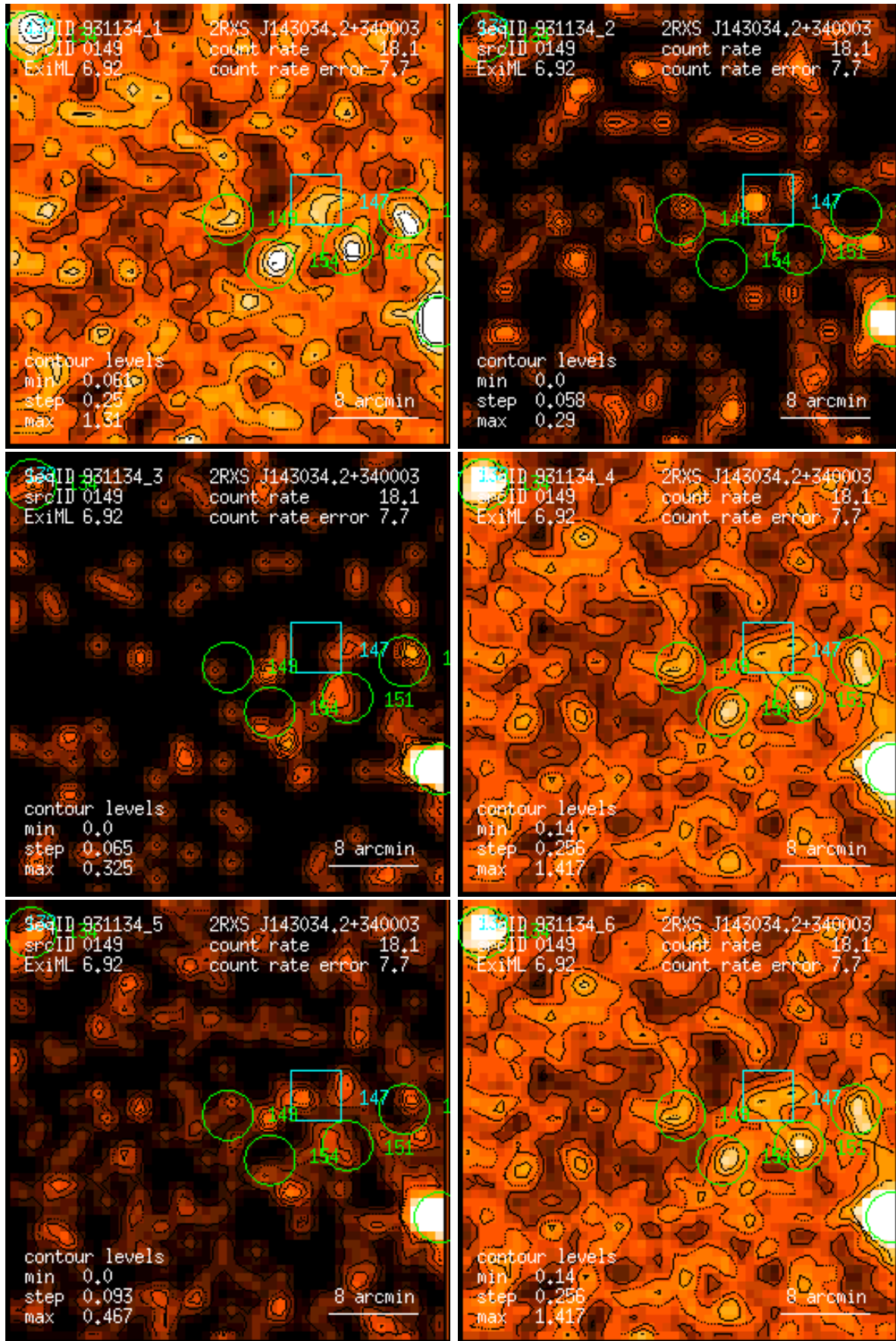
Figure 149: RASS 931134: detection 0149: band rate images, Gaussian filter: (1) PSPC channels 11 – 41, (2) 52 – 90, (3) 91 – 201, (4) 11 – 235, (5) 52 – 201, (6) 11 – 201. Broad band rates in counts/ks. Band rate contour levels in counts/ks/arcmin 2 .
