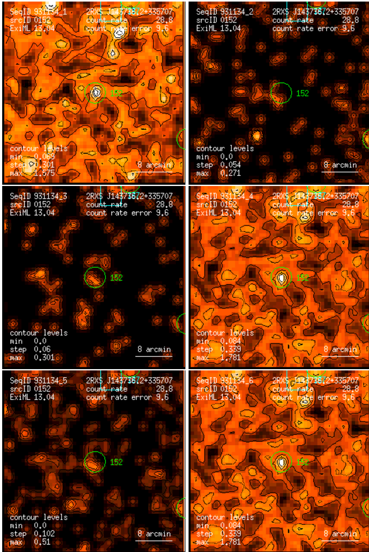
Figure 152: RASS 931134: detection 0152: band rate images, Gaussian filter: (1) PSPC channels 11 – 41, (2) 52 – 90, (3) 91 – 201, (4) 11 – 235, (5) 52 – 201, (6) 11 – 201. Broad band rates in counts/ks. Band rate contour levels in counts/ks/arcmin 2 .
