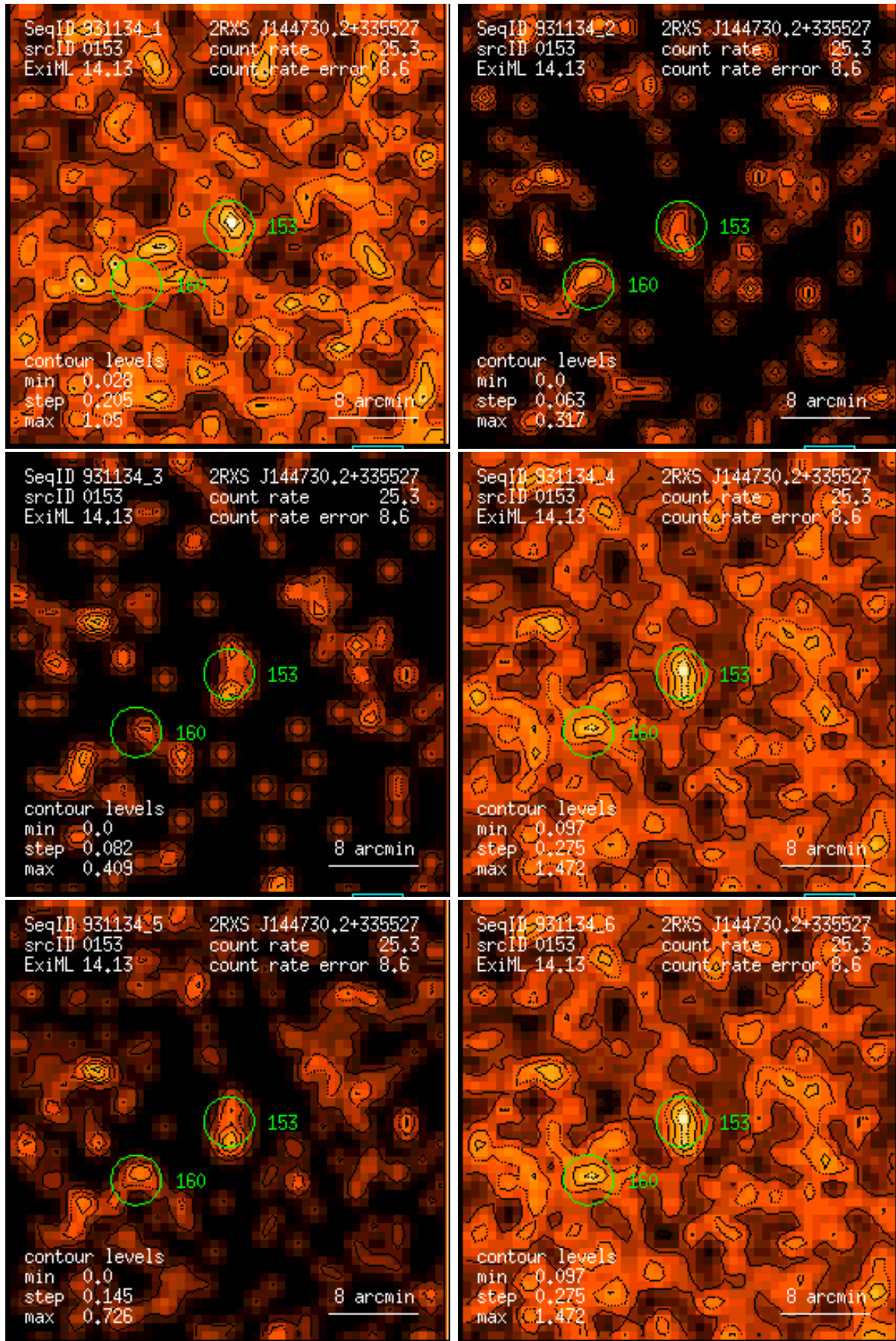
Figure 153: RASS 931134: detection 0153: band rate images, Gaussian filter: (1) PSPC channels 11 – 41, (2) 52 – 90, (3) 91 – 201, (4) 11 – 235, (5) 52 – 201, (6) 11 – 201. Broad band rates in counts/ks. Band rate contour levels in counts/ks/arcmin 2 .
