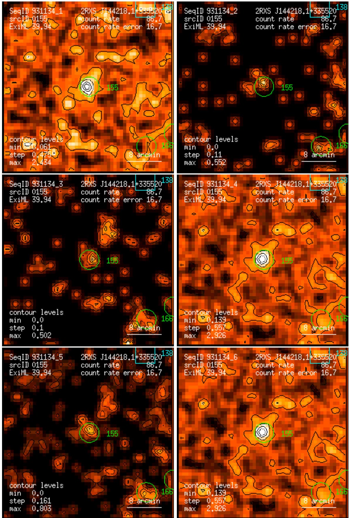
Figure 155: RASS 931134: detection 0155: band rate images, Gaussian filter: (1) PSPC channels 11 – 41, (2) 52 – 90, (3) 91 – 201, (4) 11 – 235, (5) 52 – 201, (6) 11 – 201. Broad band rates in counts/ks. Band rate contour levels in counts/ks/arcmin 2 .
