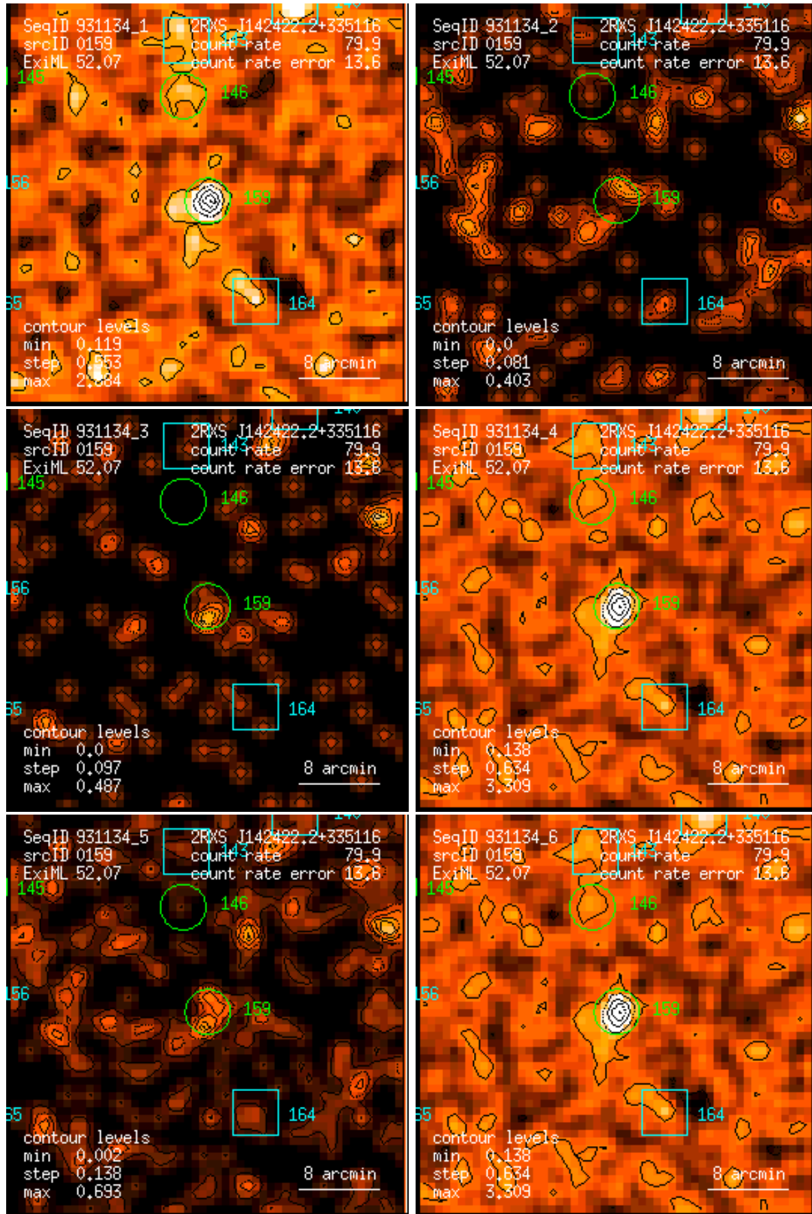
Figure 159: RASS 931134: detection 0159: band rate images, Gaussian filter: (1) PSPC channels 11 – 41, (2) 52 – 90, (3) 91 – 201, (4) 11 – 235, (5) 52 – 201, (6) 11 – 201. Broad band rates in counts/ks. Band rate contour levels in counts/ks/arcmin 2 .
