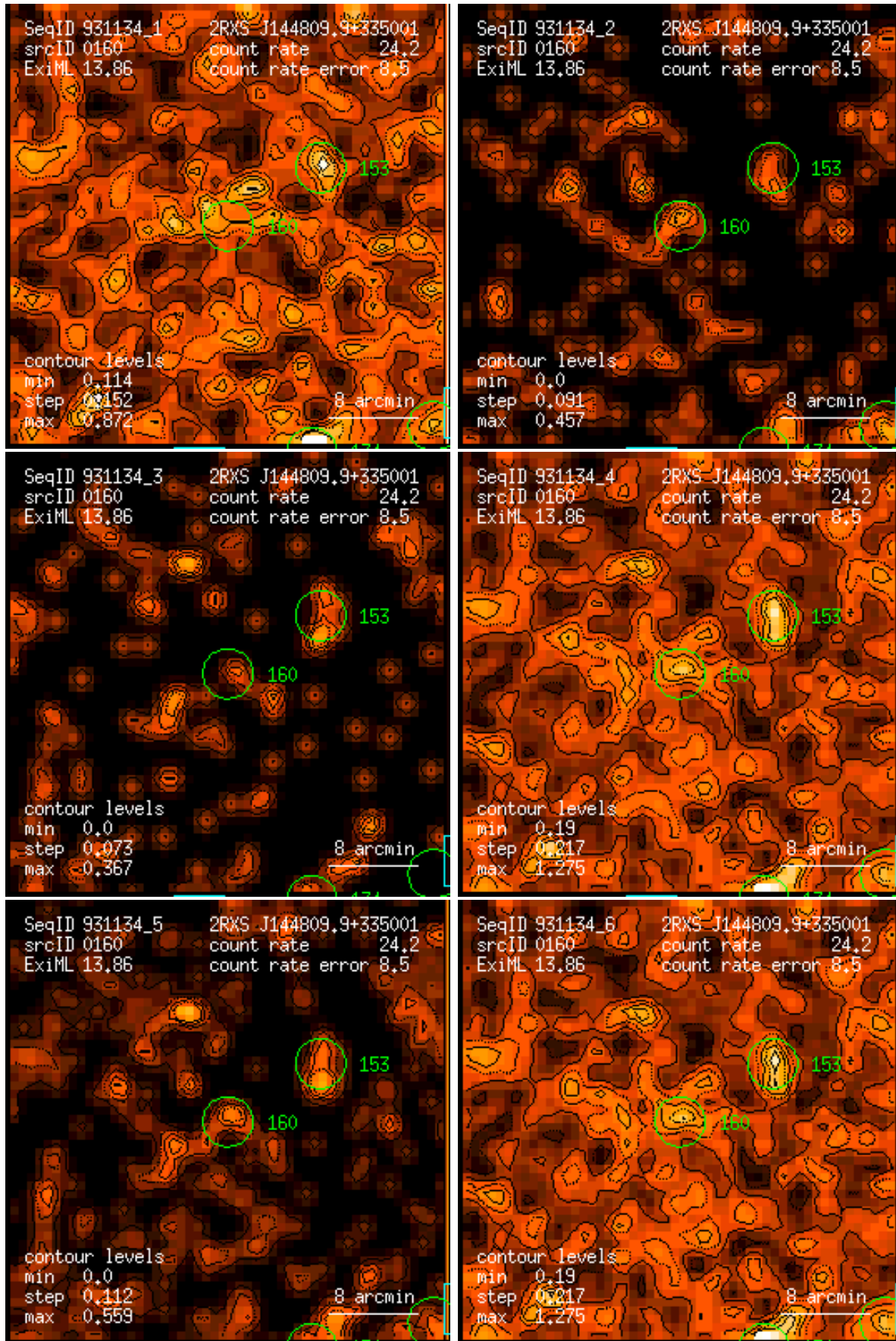
Figure 160: RASS 931134: detection 0160: band rate images, Gaussian filter: (1) PSPC channels 11 – 41, (2) 52 – 90, (3) 91 – 201, (4) 11 – 235, (5) 52 – 201, (6) 11 – 201. Broad band rates in counts/ks. Band rate contour levels in counts/ks/arcmin 2 .
