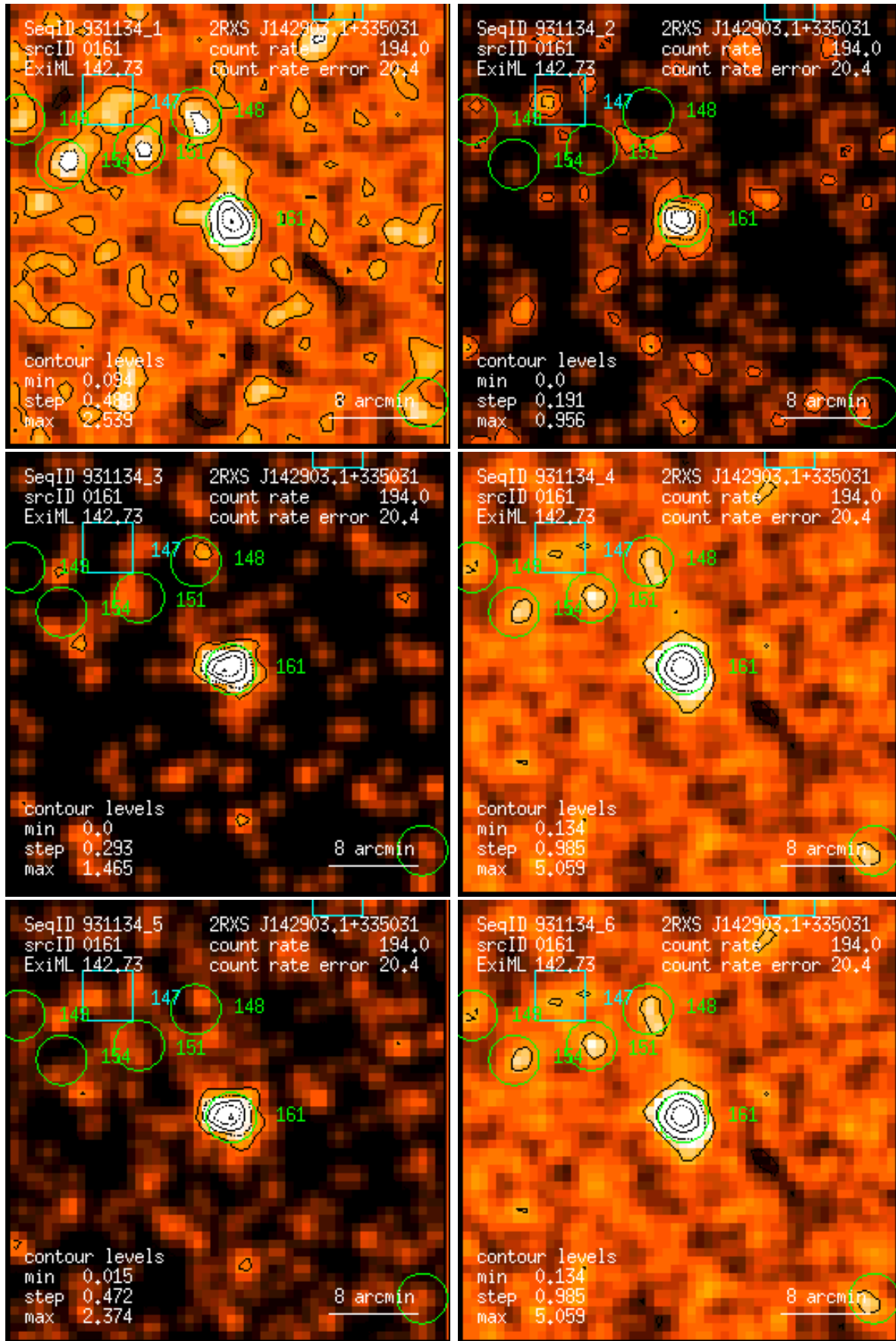
Figure 161: RASS 931134: detection 0161: band rate images, Gaussian filter: (1) PSPC channels 11 – 41, (2) 52 – 90, (3) 91 – 201, (4) 11 – 235, (5) 52 – 201, (6) 11 – 201. Broad band rates in counts/ks. Band rate contour levels in counts/ks/arcmin 2 .
