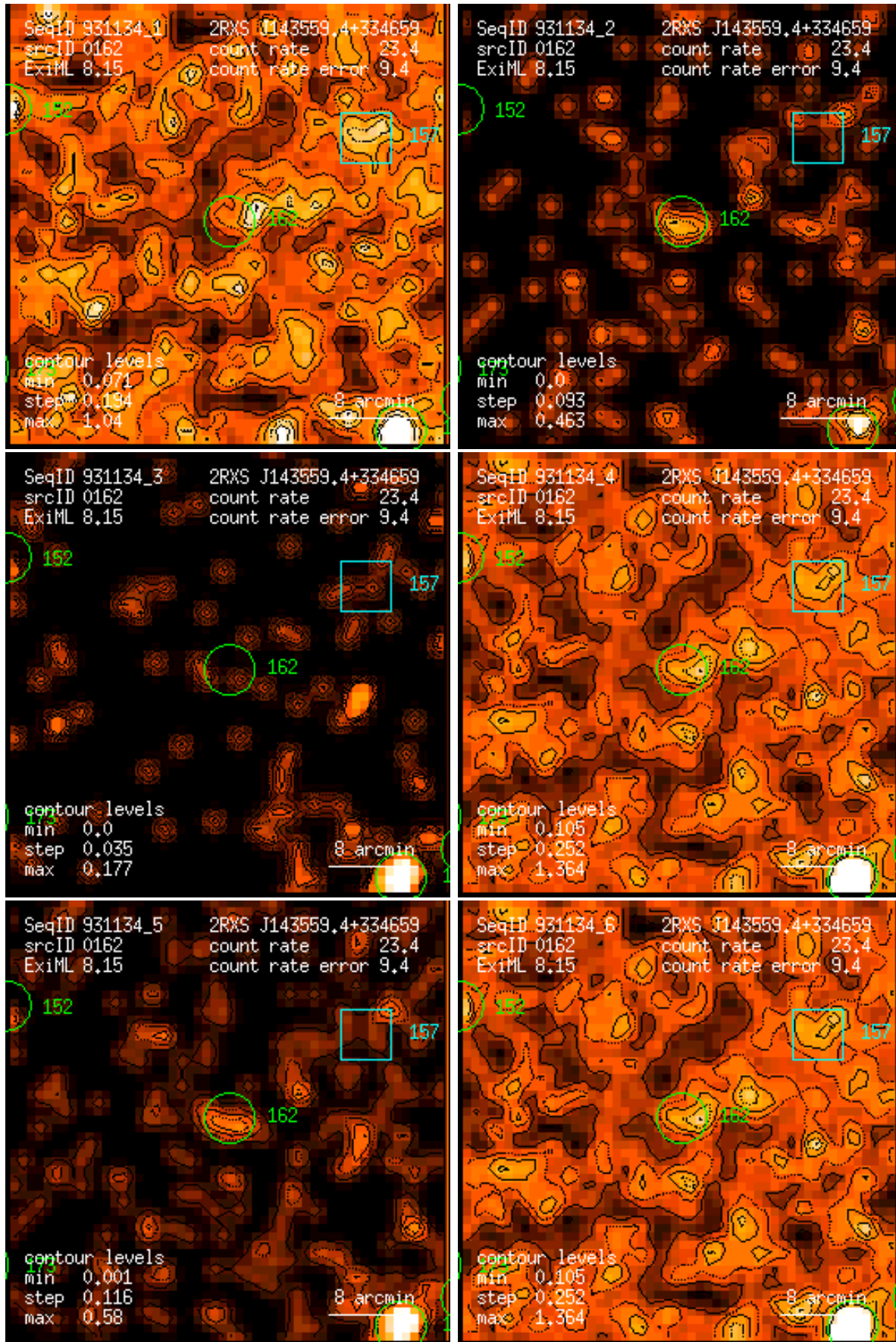
Figure 162: RASS 931134: detection 0162: band rate images, Gaussian filter: (1) PSPC channels 11 – 41, (2) 52 – 90, (3) 91 – 201, (4) 11 – 235, (5) 52 – 201, (6) 11 – 201. Broad band rates in counts/ks. Band rate contour levels in counts/ks/arcmin 2 .
