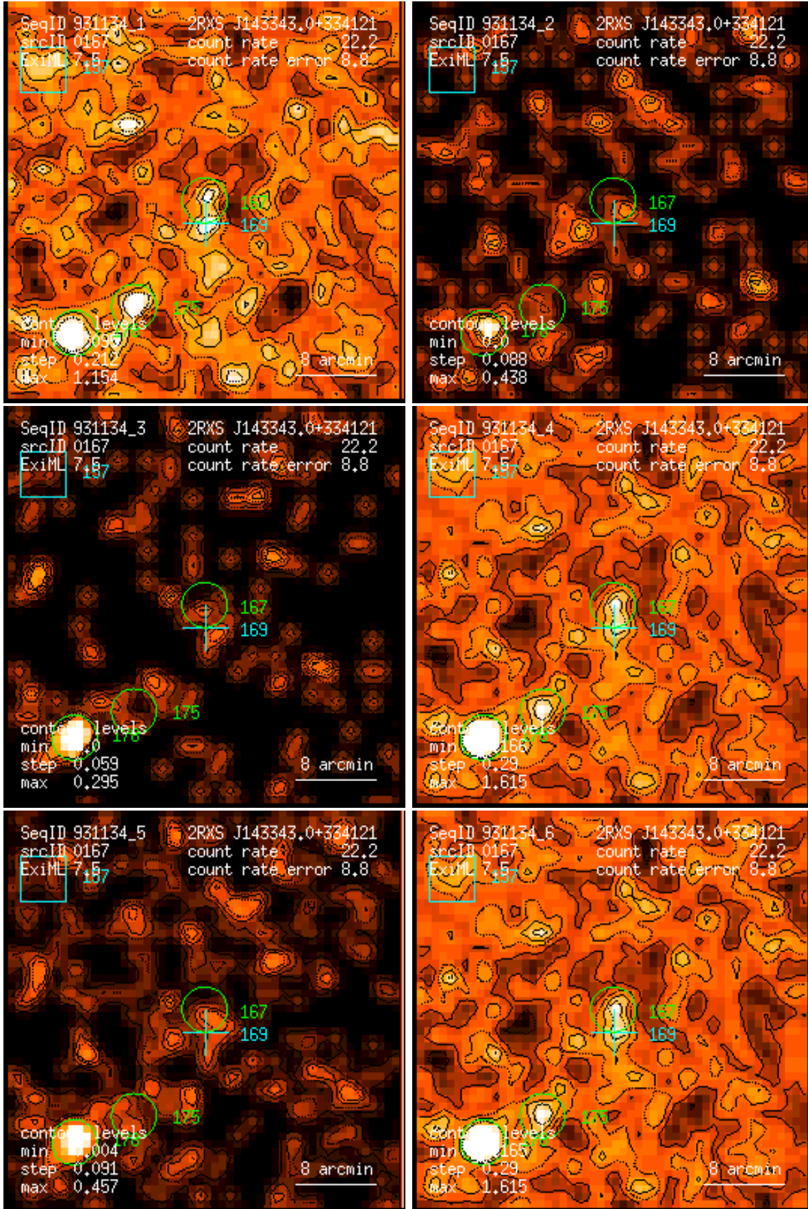
Figure 167: RASS 931134: detection 0167: band rate images, Gaussian filter: (1) PSPC channels 11 – 41, (2) 52 – 90, (3) 91 – 201, (4) 11 – 235, (5) 52 – 201, (6) 11 – 201. Broad band rates in counts/ks. Band rate contour levels in counts/ks/arcmin 2 .
