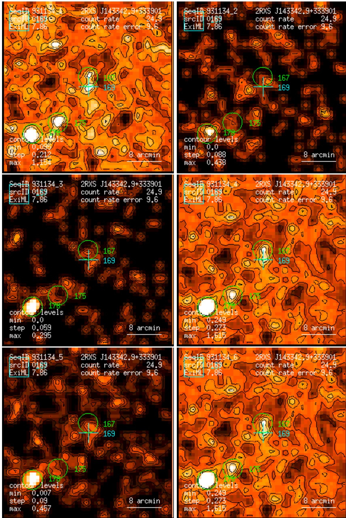
Figure 169: RASS 931134: detection 0169: band rate images, Gaussian filter: (1) PSPC channels 11 – 41, (2) 52 – 90, (3) 91 – 201, (4) 11 – 235, (5) 52 – 201, (6) 11 – 201. Broad band rates in counts/ks. Band rate contour levels in counts/ks/arcmin 2 .
