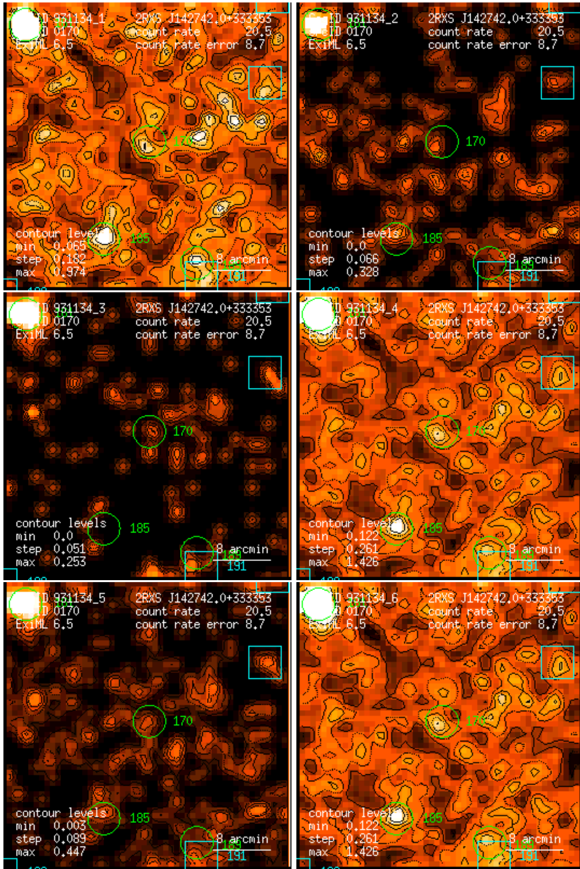
Figure 170: RASS 931134: detection 0170: band rate images, Gaussian filter: (1) PSPC channels 11 – 41, (2) 52 – 90, (3) 91 – 201, (4) 11 – 235, (5) 52 – 201, (6) 11 – 201. Broad band rates in counts/ks. Band rate contour levels in counts/ks/arcmin 2 .
