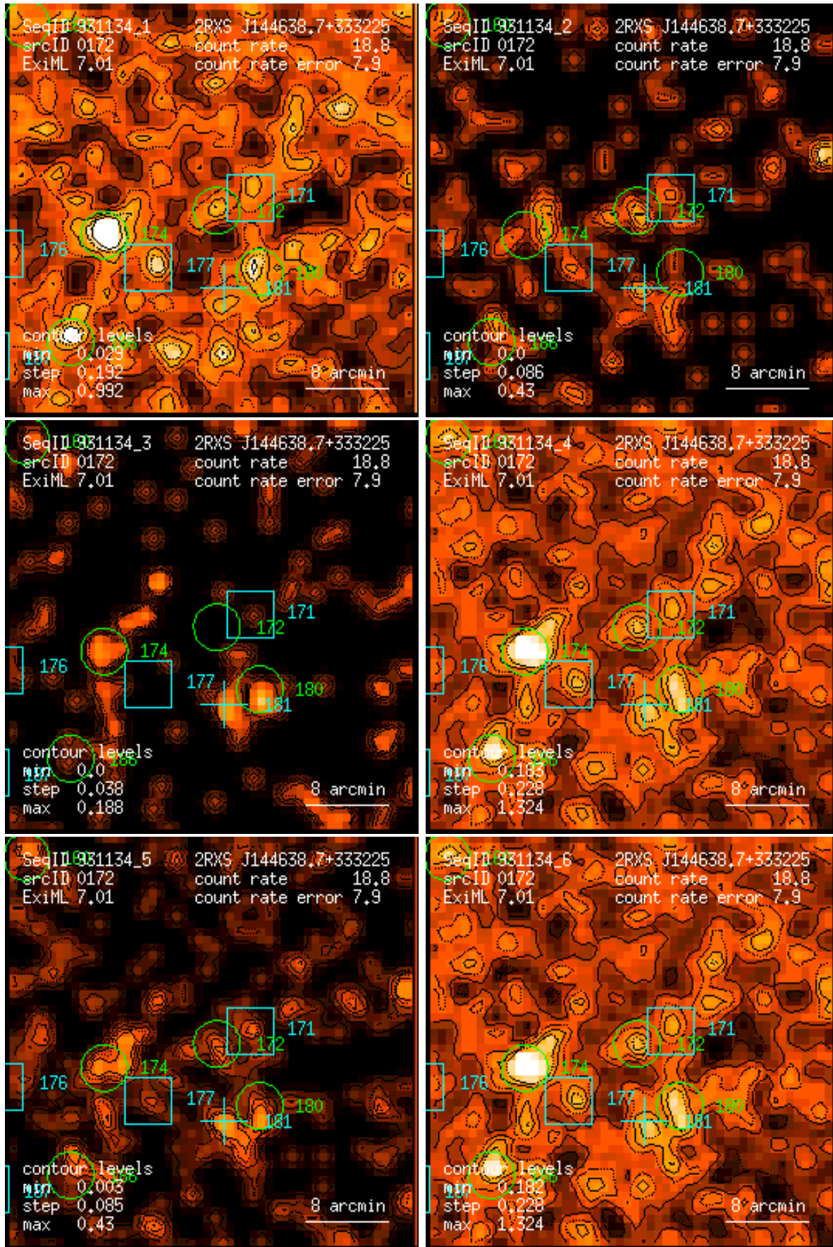
Figure 172: RASS 931134: detection 0172: band rate images, Gaussian filter: (1) PSPC channels 11 – 41, (2) 52 – 90, (3) 91 – 201, (4) 11 – 235, (5) 52 – 201, (6) 11 – 201. Broad band rates in counts/ks. Band rate contour levels in counts/ks/arcmin 2 .
