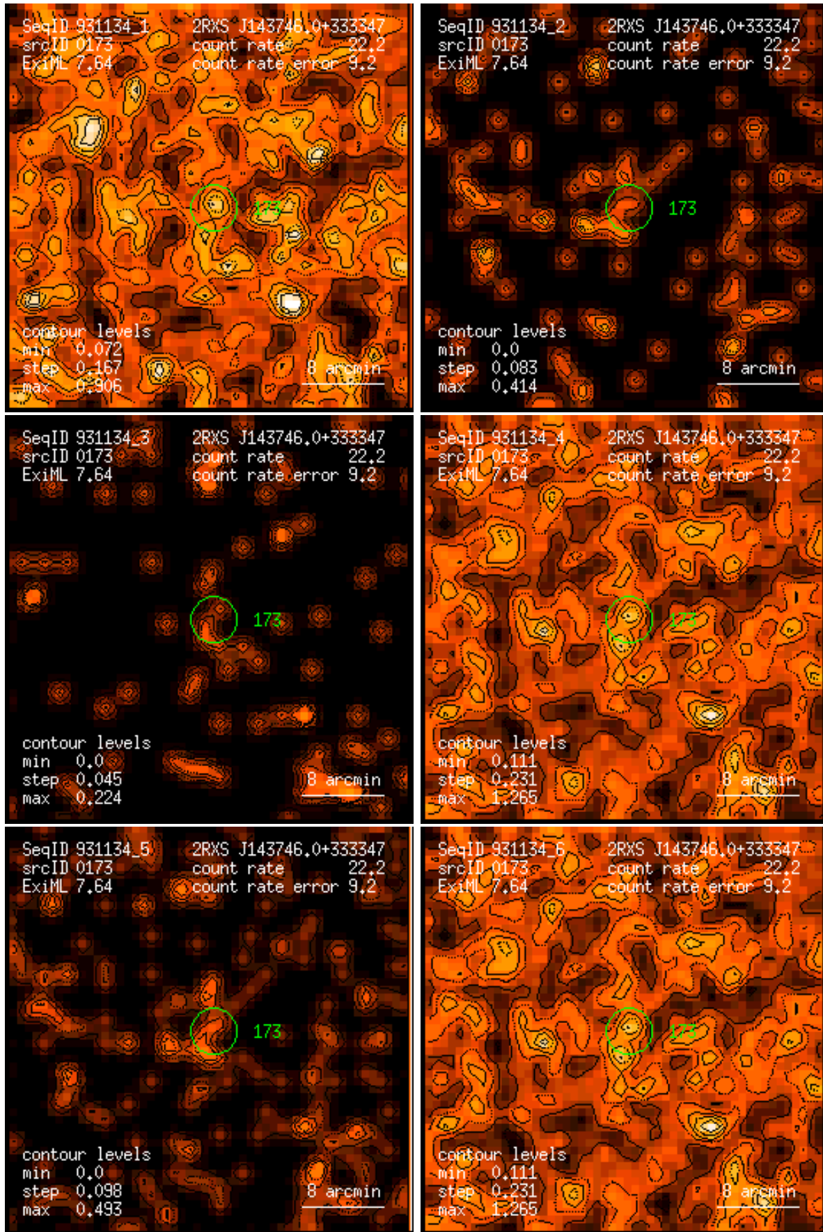
Figure 173: RASS 931134: detection 0173: band rate images, Gaussian filter: (1) PSPC channels 11 – 41, (2) 52 – 90, (3) 91 – 201, (4) 11 – 235, (5) 52 – 201, (6) 11 – 201. Broad band rates in counts/ks. Band rate contour levels in counts/ks/arcmin 2 .
