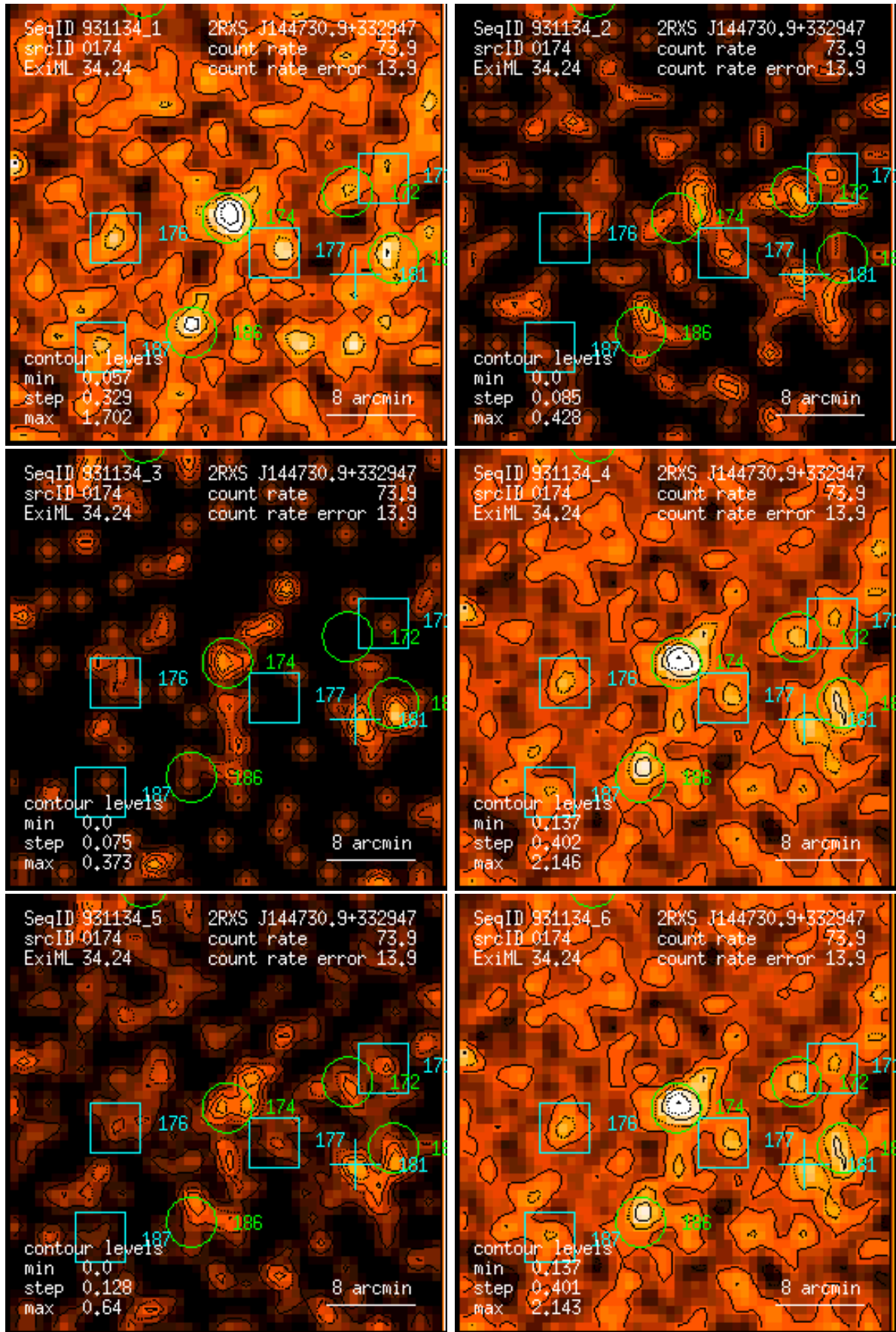
Figure 174: RASS 931134: detection 0174: band rate images, Gaussian filter: (1) PSPC channels 11 – 41, (2) 52 – 90, (3) 91 – 201, (4) 11 – 235, (5) 52 – 201, (6) 11 – 201. Broad band rates in counts/ks. Band rate contour levels in counts/ks/arcmin 2 .
