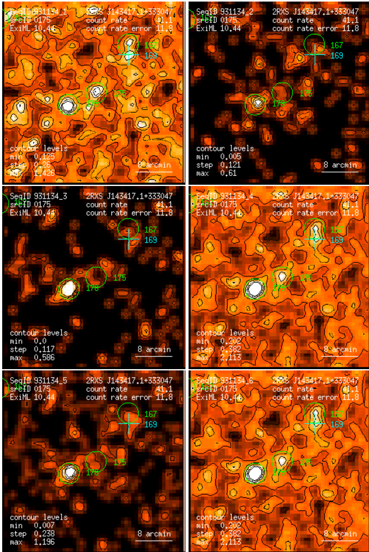
Figure 175: RASS 931134: detection 0175: band rate images, Gaussian filter: (1) PSPC channels 11 – 41, (2) 52 – 90, (3) 91 – 201, (4) 11 – 235, (5) 52 – 201, (6) 11 – 201. Broad band rates in counts/ks. Band rate contour levels in counts/ks/arcmin 2 .
