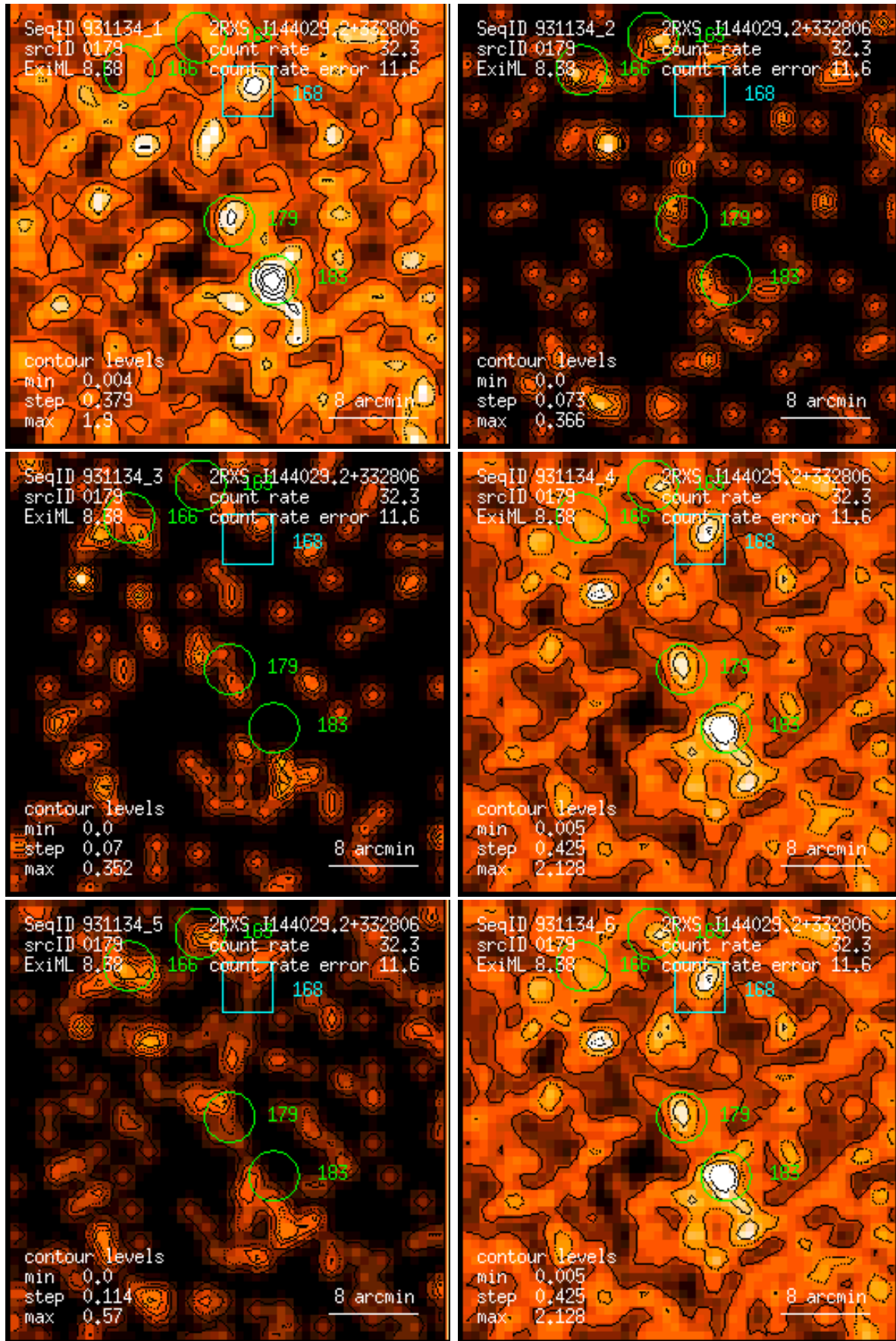
Figure 179: RASS 931134: detection 0179: band rate images, Gaussian filter: (1) PSPC channels 11 – 41, (2) 52 – 90, (3) 91 – 201, (4) 11 – 235, (5) 52 – 201, (6) 11 – 201. Broad band rates in counts/ks. Band rate contour levels in counts/ks/arcmin 2 .
