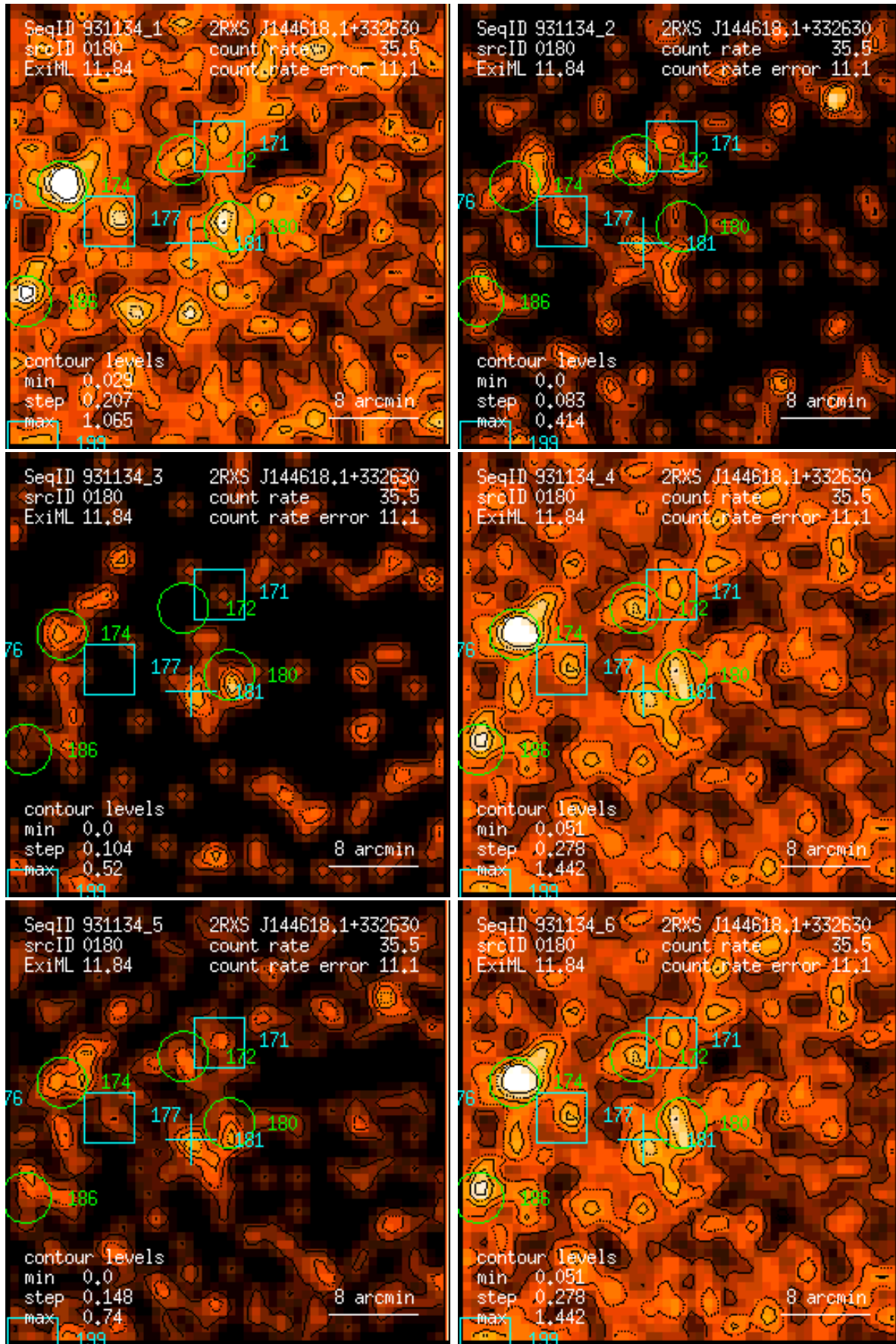
Figure 180: RASS 931134: detection 0180: band rate images, Gaussian filter: (1) PSPC channels 11 – 41, (2) 52 – 90, (3) 91 – 201, (4) 11 – 235, (5) 52 – 201, (6) 11 – 201. Broad band rates in counts/ks. Band rate contour levels in counts/ks/arcmin 2 .
