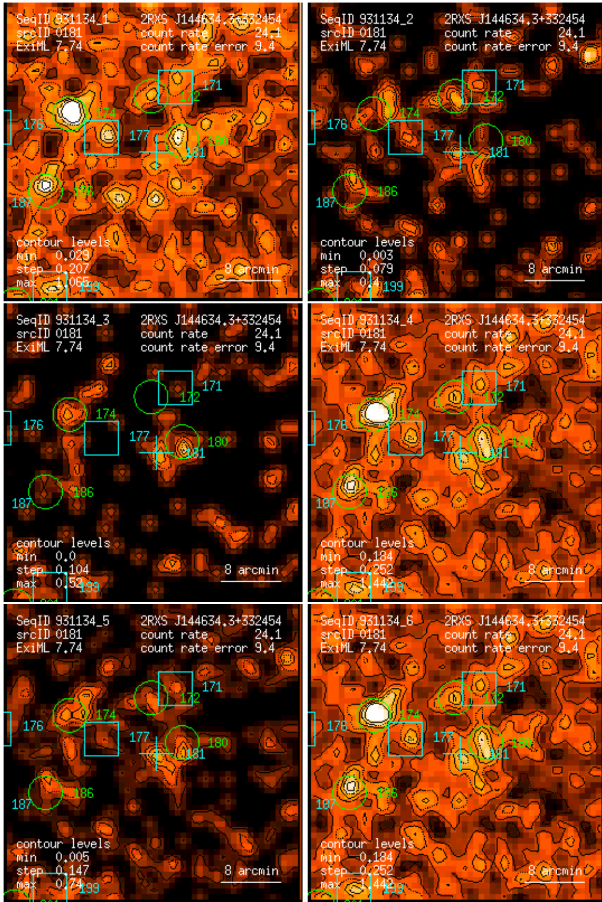
Figure 181: RASS 931134: detection 0181: band rate images, Gaussian filter: (1) PSPC channels 11 – 41, (2) 52 – 90, (3) 91 – 201, (4) 11 – 235, (5) 52 – 201, (6) 11 – 201. Broad band rates in counts/ks. Band rate contour levels in counts/ks/arcmin 2 .
