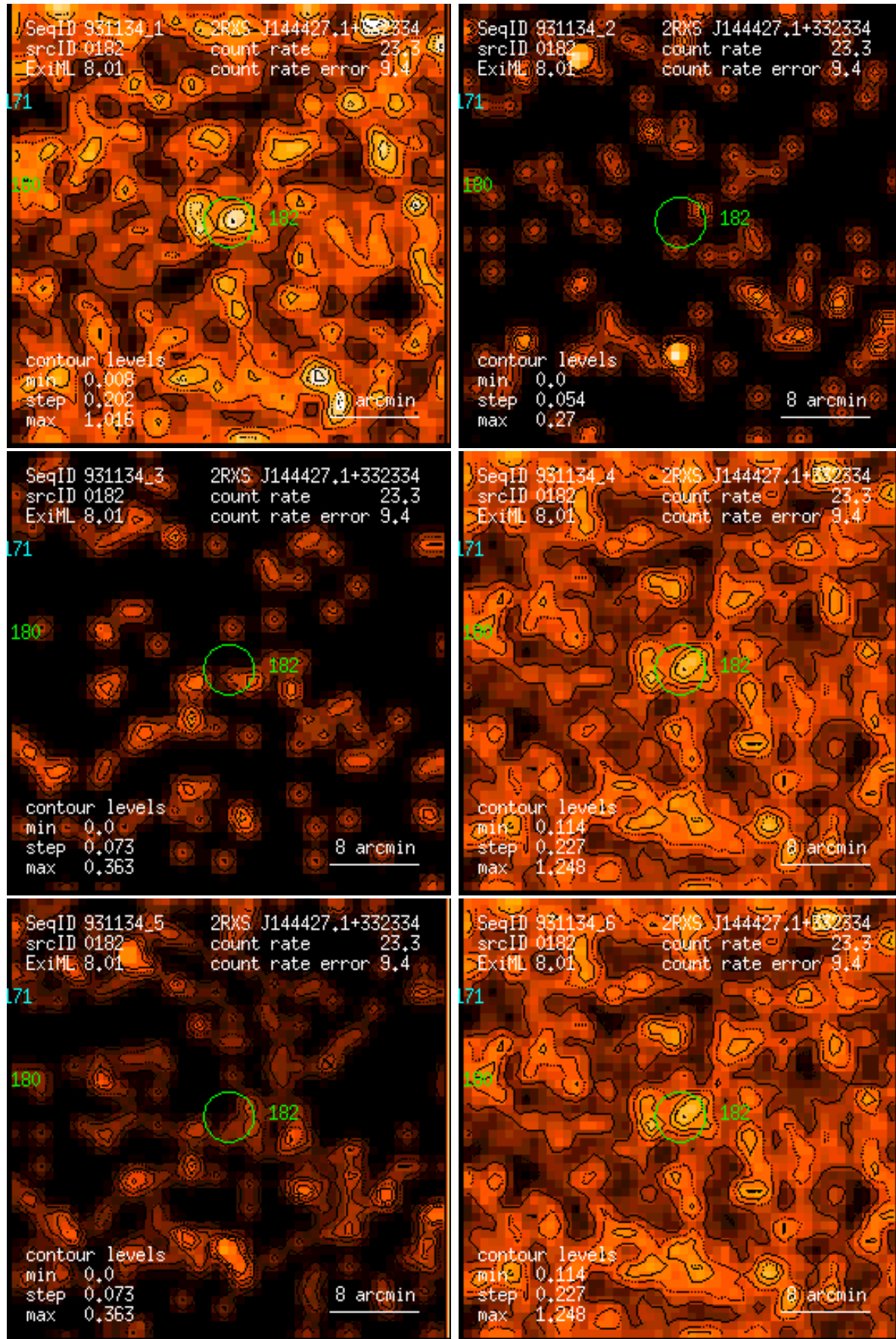
Figure 182: RASS 931134: detection 0182: band rate images, Gaussian filter: (1) PSPC channels 11 – 41, (2) 52 – 90, (3) 91 – 201, (4) 11 – 235, (5) 52 – 201, (6) 11 – 201. Broad band rates in counts/ks. Band rate contour levels in counts/ks/arcmin 2 .
