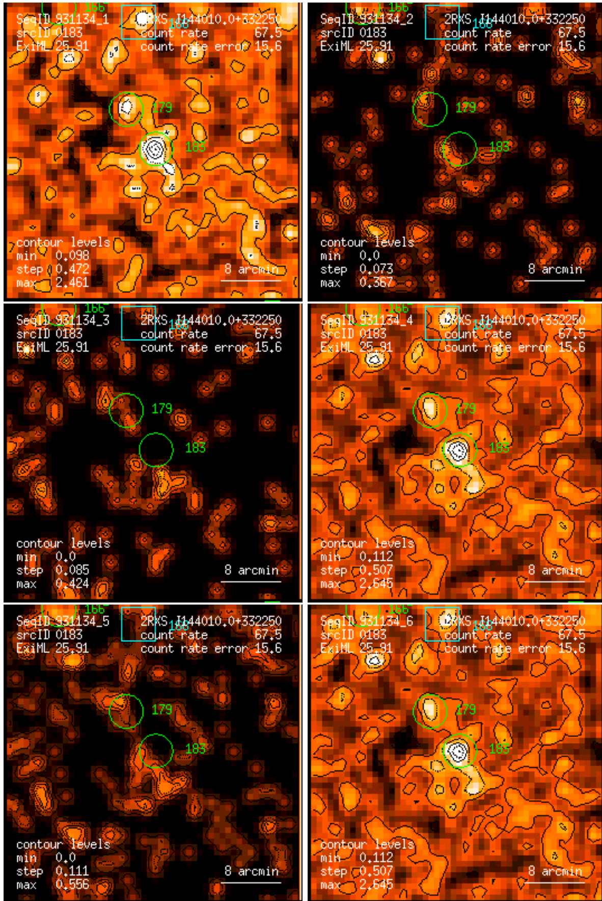
Figure 183: RASS 931134: detection 0183: band rate images, Gaussian filter: (1) PSPC channels 11 – 41, (2) 52 – 90, (3) 91 – 201, (4) 11 – 235, (5) 52 – 201, (6) 11 – 201. Broad band rates in counts/ks. Band rate contour levels in counts/ks/arcmin 2 .
