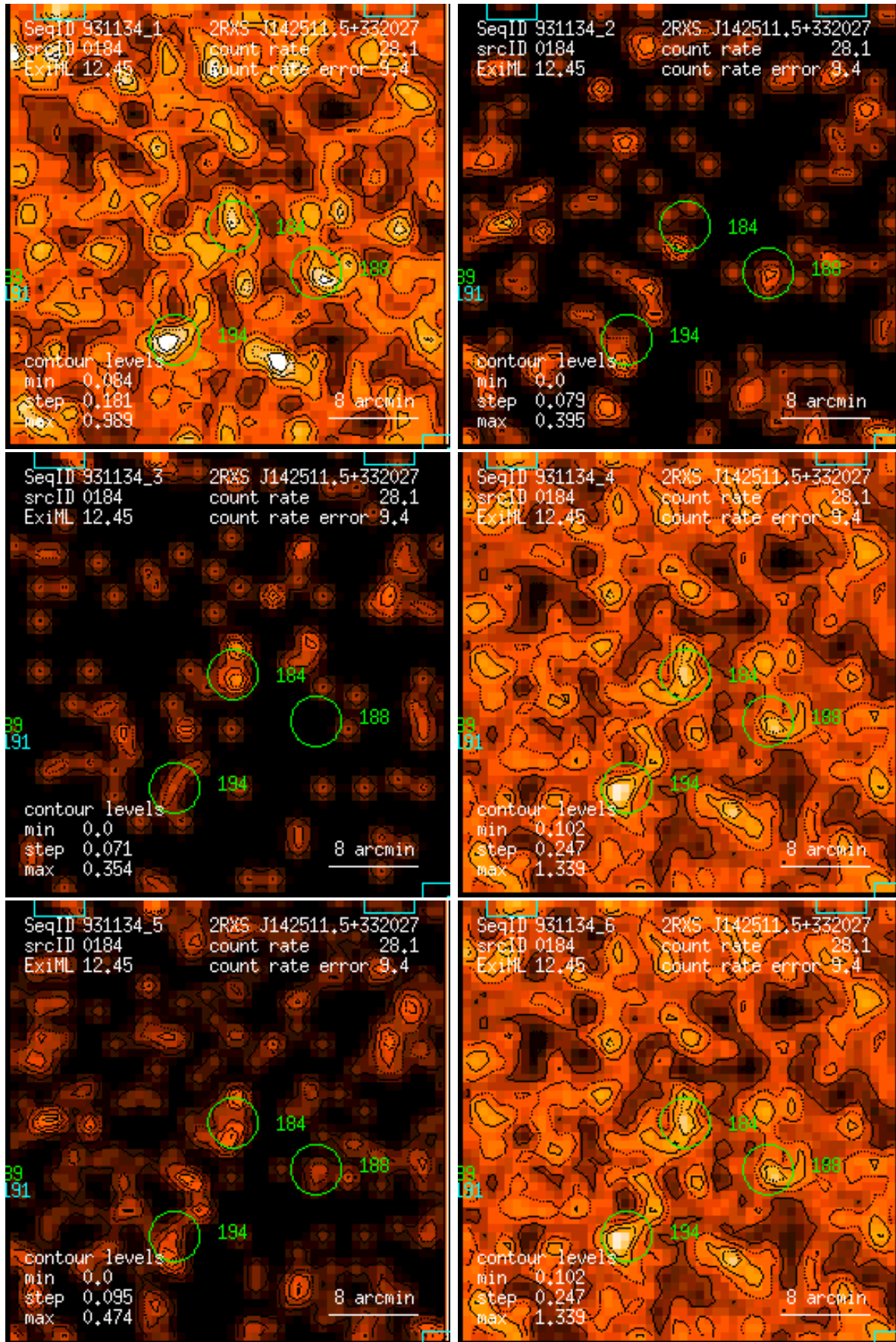
Figure 184: RASS 931134: detection 0184: band rate images, Gaussian filter: (1) PSPC channels 11 – 41, (2) 52 – 90, (3) 91 – 201, (4) 11 – 235, (5) 52 – 201, (6) 11 – 201. Broad band rates in counts/ks. Band rate contour levels in counts/ks/arcmin 2 .
