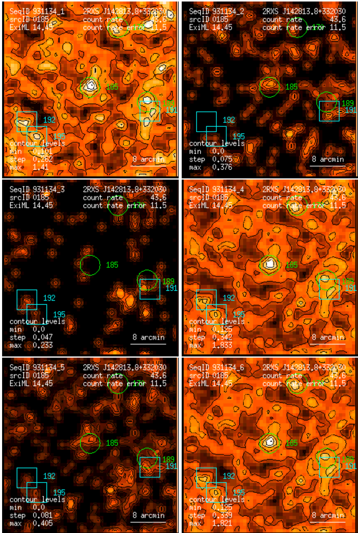
Figure 185: RASS 931134: detection 0185: band rate images, Gaussian filter: (1) PSPC channels 11 – 41, (2) 52 – 90, (3) 91 – 201, (4) 11 – 235, (5) 52 – 201, (6) 11 – 201. Broad band rates in counts/ks. Band rate contour levels in counts/ks/arcmin 2 .
