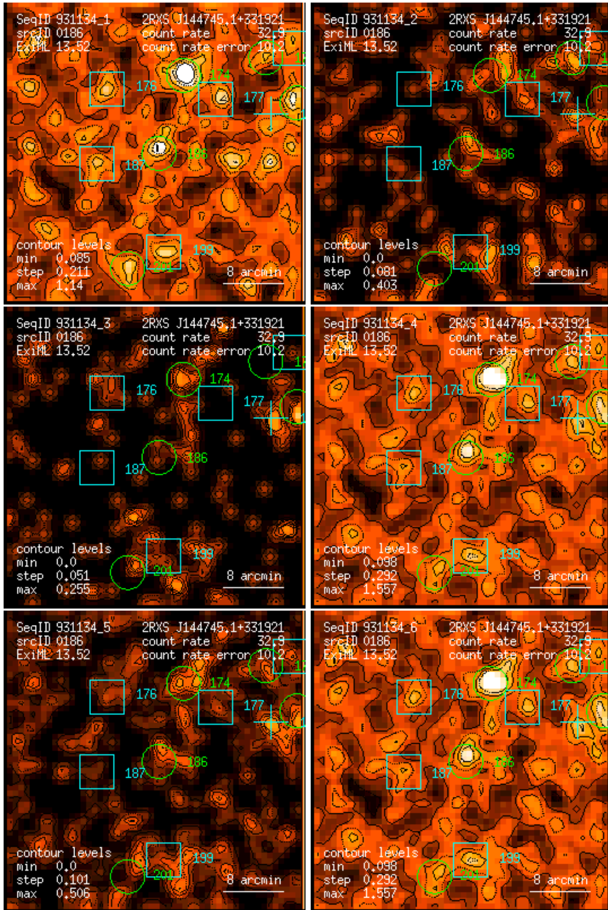
Figure 186: RASS 931134: detection 0186: band rate images, Gaussian filter: (1) PSPC channels 11 – 41, (2) 52 – 90, (3) 91 – 201, (4) 11 – 235, (5) 52 – 201, (6) 11 – 201. Broad band rates in counts/ks. Band rate contour levels in counts/ks/arcmin 2 .
