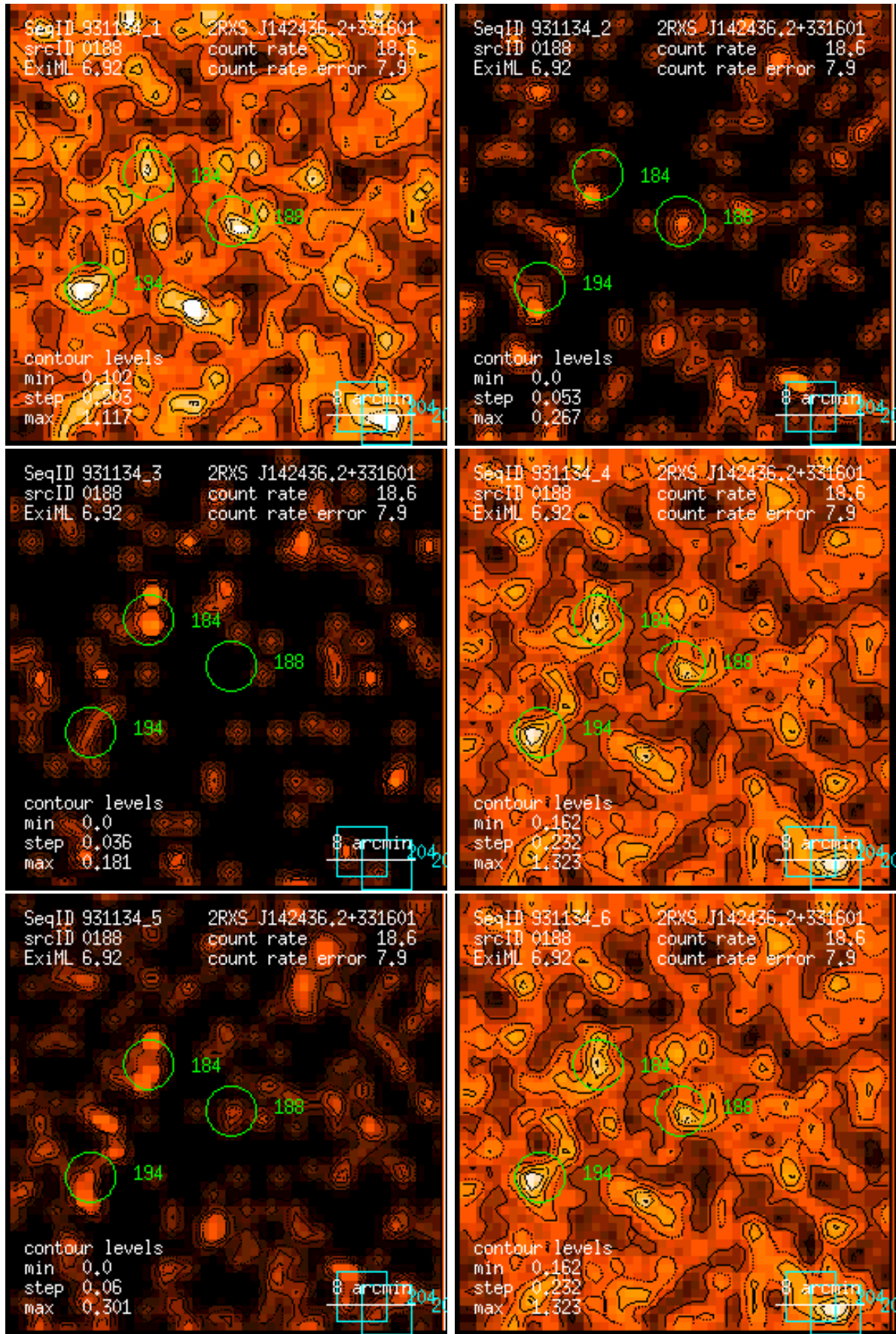
Figure 188: RASS 931134: detection 0188: band rate images, Gaussian filter: (1) PSPC channels 11 – 41, (2) 52 – 90, (3) 91 – 201, (4) 11 – 235, (5) 52 – 201, (6) 11 – 201. Broad band rates in counts/ks. Band rate contour levels in counts/ks/arcmin 2 .
