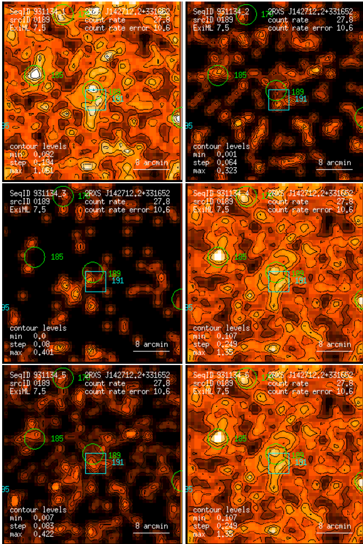
Figure 189: RASS 931134: detection 0189: band rate images, Gaussian filter: (1) PSPC channels 11 – 41, (2) 52 – 90, (3) 91 – 201, (4) 11 – 235, (5) 52 – 201, (6) 11 – 201. Broad band rates in counts/ks. Band rate contour levels in counts/ks/arcmin 2 .
