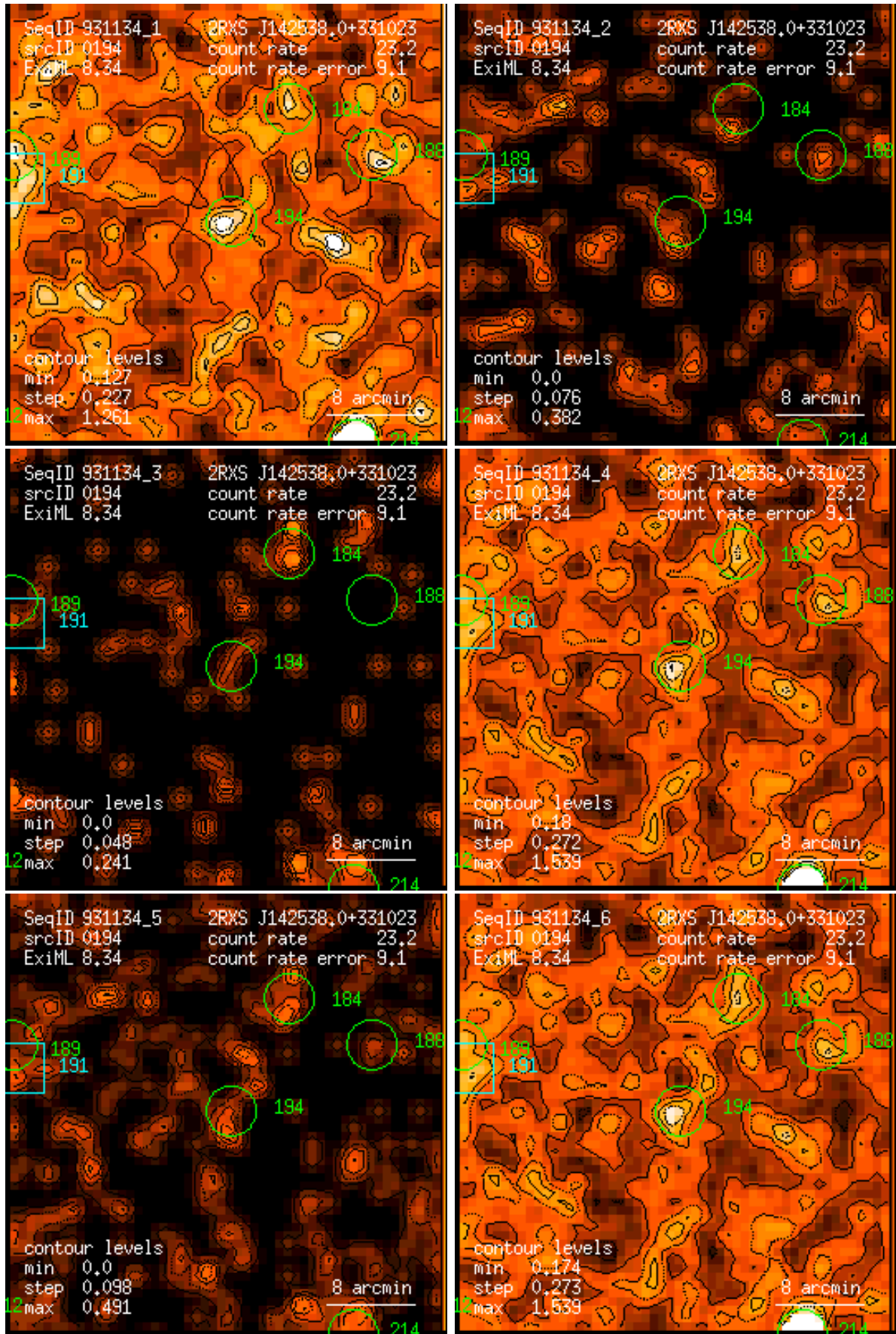
Figure 194: RASS 931134: detection 0194: band rate images, Gaussian filter: (1) PSPC channels 11 – 41, (2) 52 – 90, (3) 91 – 201, (4) 11 – 235, (5) 52 – 201, (6) 11 – 201. Broad band rates in counts/ks. Band rate contour levels in counts/ks/arcmin 2 .
