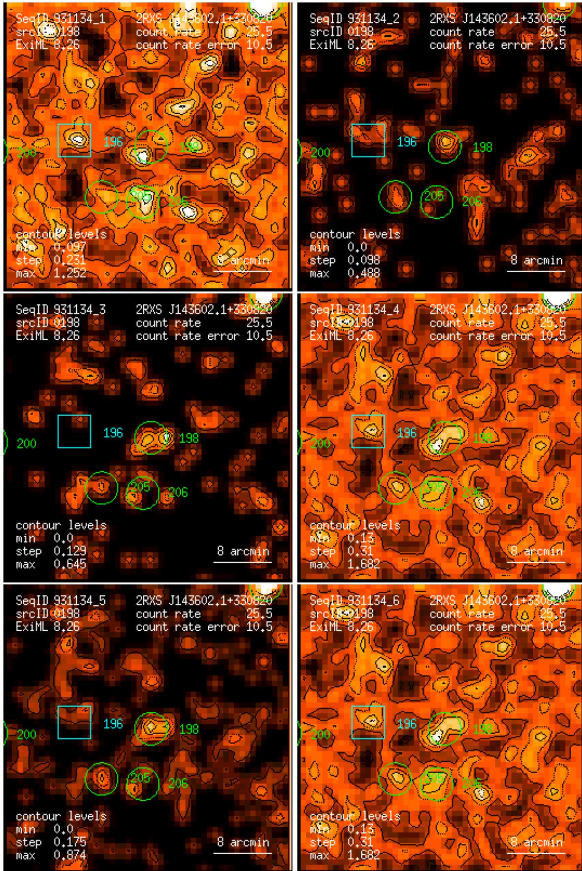
Figure 198: RASS 931134: detection 0198: band rate images, Gaussian filter: (1) PSPC channels 11 – 41, (2) 52 – 90, (3) 91 – 201, (4) 11 – 235, (5) 52 – 201, (6) 11 – 201. Broad band rates in counts/ks. Band rate contour levels in counts/ks/arcmin 2 .
