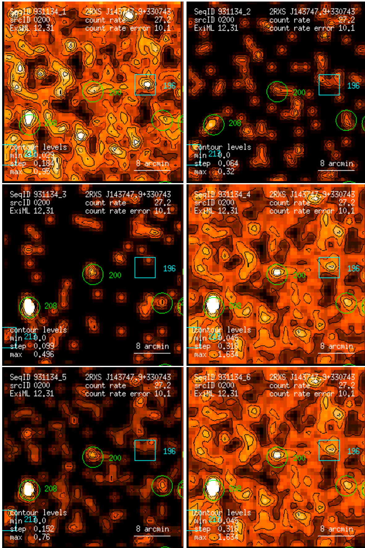
Figure 200: RASS 931134: detection 0200: band rate images, Gaussian filter: (1) PSPC channels 11 – 41, (2) 52 – 90, (3) 91 – 201, (4) 11 – 235, (5) 52 – 201, (6) 11 – 201. Broad band rates in counts/ks. Band rate contour levels in counts/ks/arcmin 2 .
