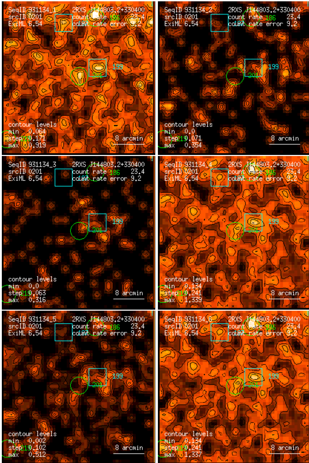
Figure 201: RASS 931134: detection 0201: band rate images, Gaussian filter: (1) PSPC channels 11 – 41, (2) 52 – 90, (3) 91 – 201, (4) 11 – 235, (5) 52 – 201, (6) 11 – 201. Broad band rates in counts/ks. Band rate contour levels in counts/ks/arcmin 2 .
