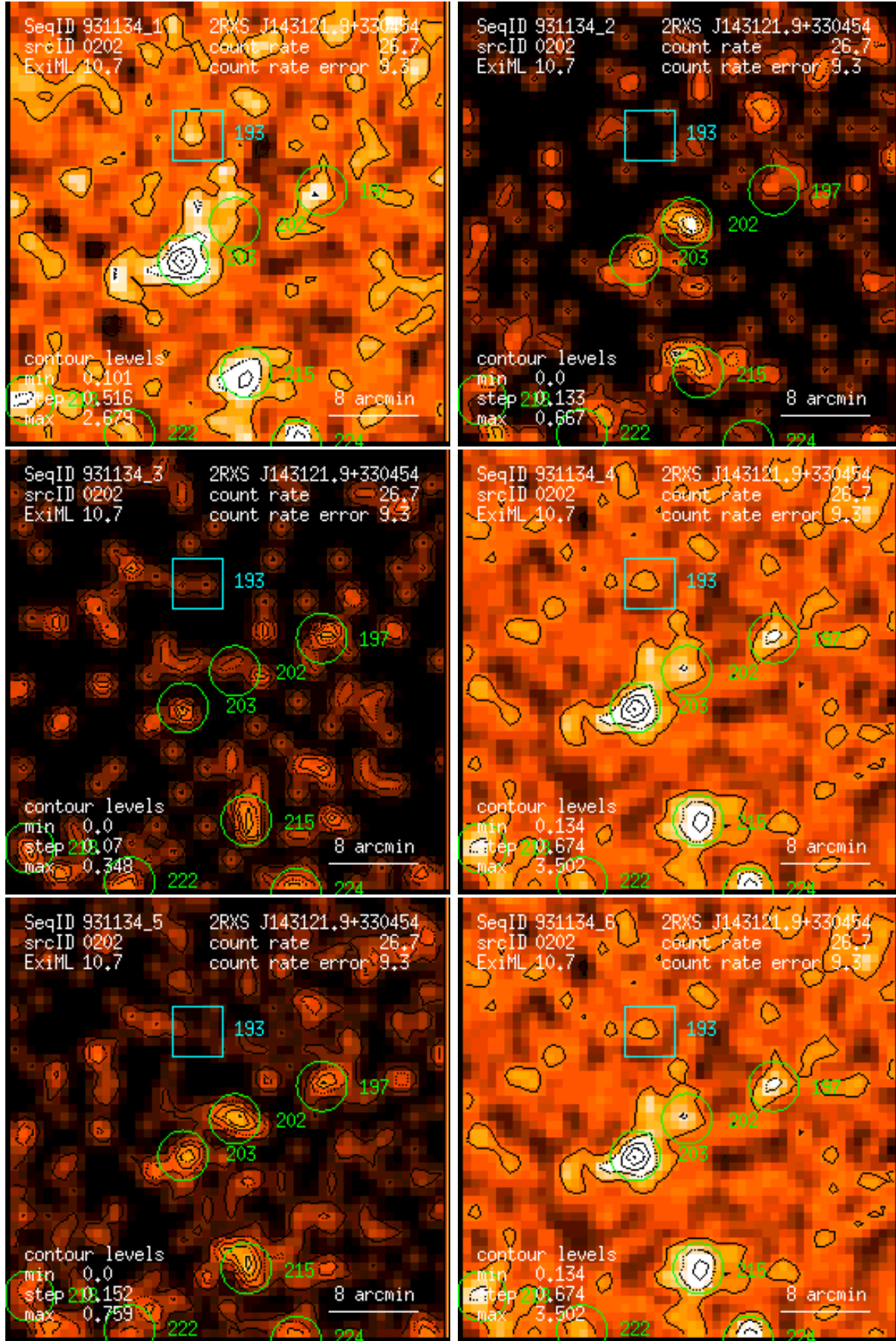
Figure 202: RASS 931134: detection 0202: band rate images, Gaussian filter: (1) PSPC channels 11 – 41, (2) 52 – 90, (3) 91 – 201, (4) 11 – 235, (5) 52 – 201, (6) 11 – 201. Broad band rates in counts/ks. Band rate contour levels in counts/ks/arcmin 2 .
