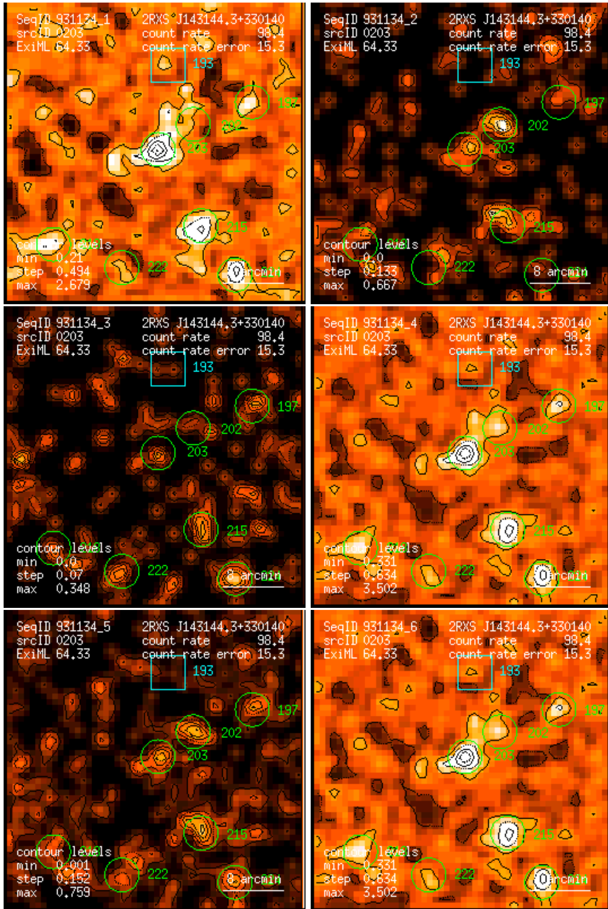
Figure 203: RASS 931134: detection 0203: band rate images, Gaussian filter: (1) PSPC channels 11 – 41, (2) 52 – 90, (3) 91 – 201, (4) 11 – 235, (5) 52 – 201, (6) 11 – 201. Broad band rates in counts/ks. Band rate contour levels in counts/ks/arcmin 2 .
