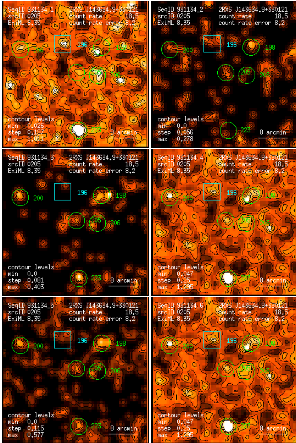
Figure 205: RASS 931134: detection 0205: band rate images, Gaussian filter: (1) PSPC channels 11 – 41, (2) 52 – 90, (3) 91 – 201, (4) 11 – 235, (5) 52 – 201, (6) 11 – 201. Broad band rates in counts/ks. Band rate contour levels in counts/ks/arcmin 2 .
