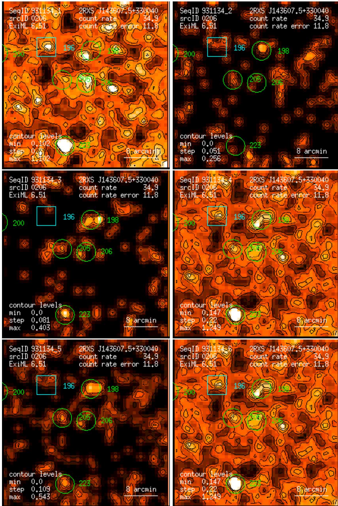
Figure 206: RASS 931134: detection 0206: band rate images, Gaussian filter: (1) PSPC channels 11 – 41, (2) 52 – 90, (3) 91 – 201, (4) 11 – 235, (5) 52 – 201, (6) 11 – 201. Broad band rates in counts/ks. Band rate contour levels in counts/ks/arcmin 2 .
