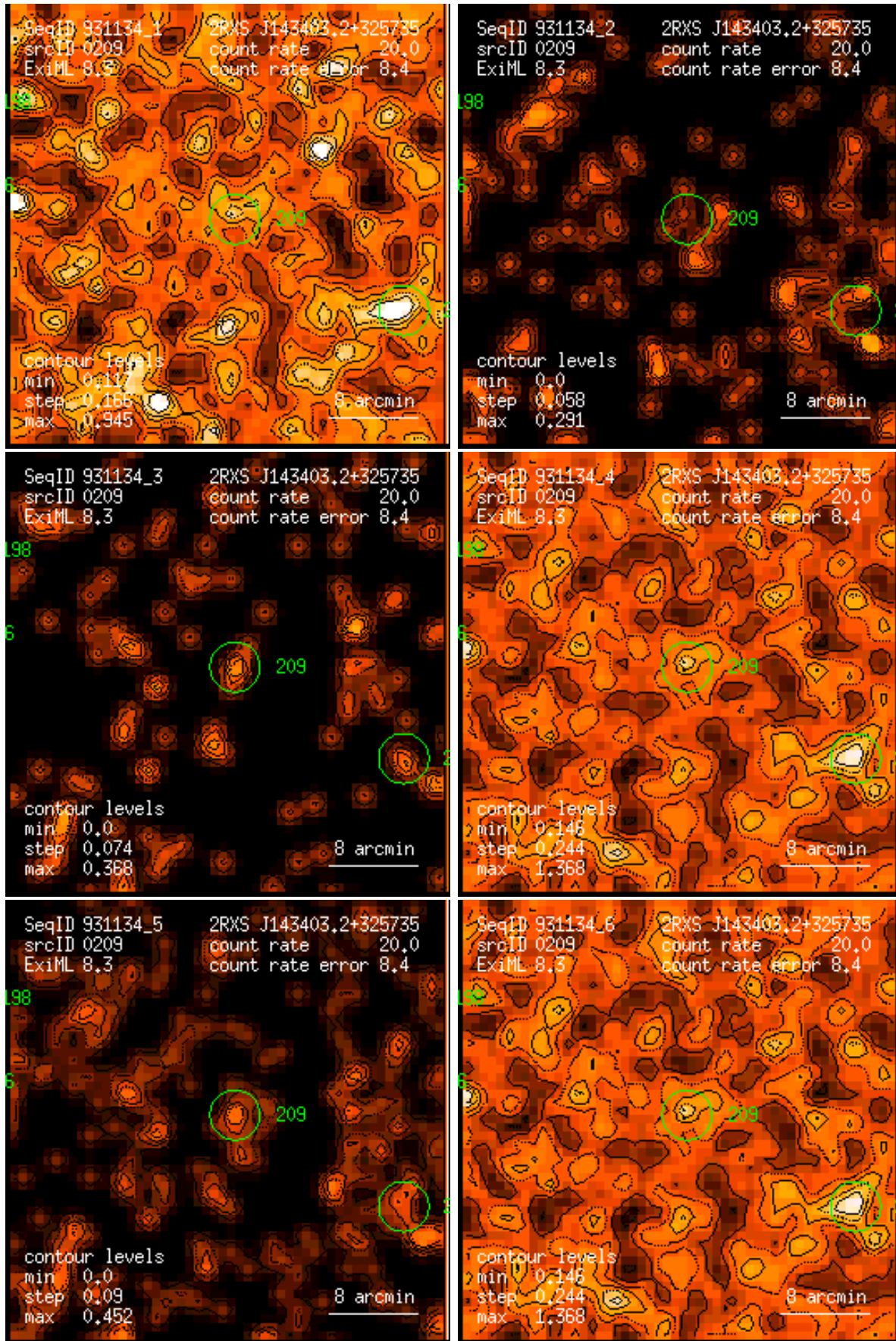
Figure 209: RASS 931134: detection 0209: band rate images, Gaussian filter: (1) PSPC channels 11 – 41, (2) 52 – 90, (3) 91 – 201, (4) 11 – 235, (5) 52 – 201, (6) 11 – 201. Broad band rates in counts/ks. Band rate contour levels in counts/ks/arcmin 2 .
