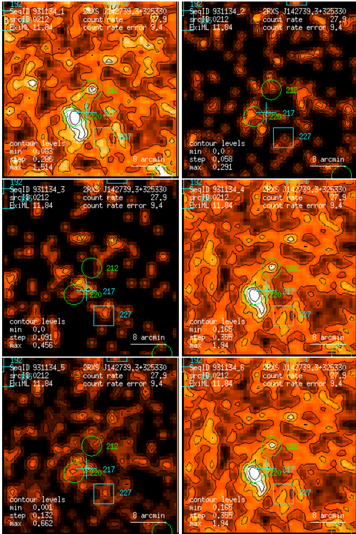
Figure 212: RASS 931134: detection 0212: band rate images, Gaussian filter: (1) PSPC channels 11 – 41, (2) 52 – 90, (3) 91 – 201, (4) 11 – 235, (5) 52 – 201, (6) 11 – 201. Broad band rates in counts/ks. Band rate contour levels in counts/ks/arcmin 2 .
